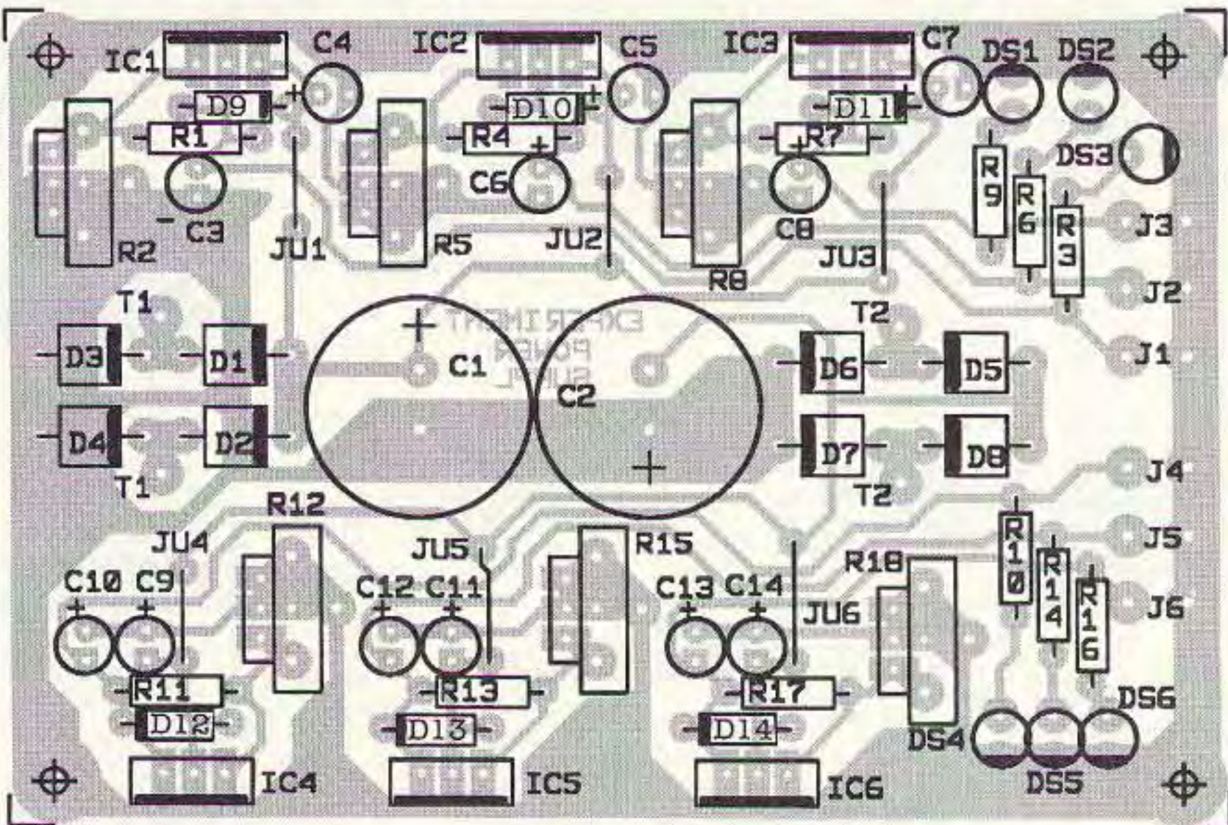
Figure A. Corrected parts placement diagram for the Experimenter's Power Supply.
