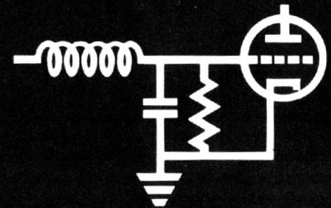
A combination RF filter is shown in Figure 17 with the recommended values.
