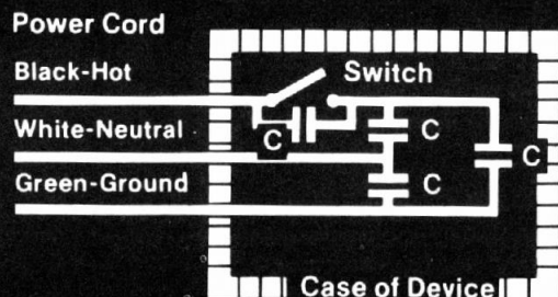
Fig. 8 C = .001 mfd., disc ceramic
