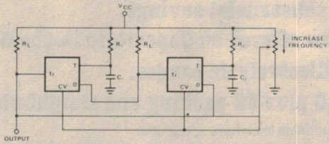
VARIABLE FREQUENCY OSCILLATOR WITH FIXED DUTY CYCLE
