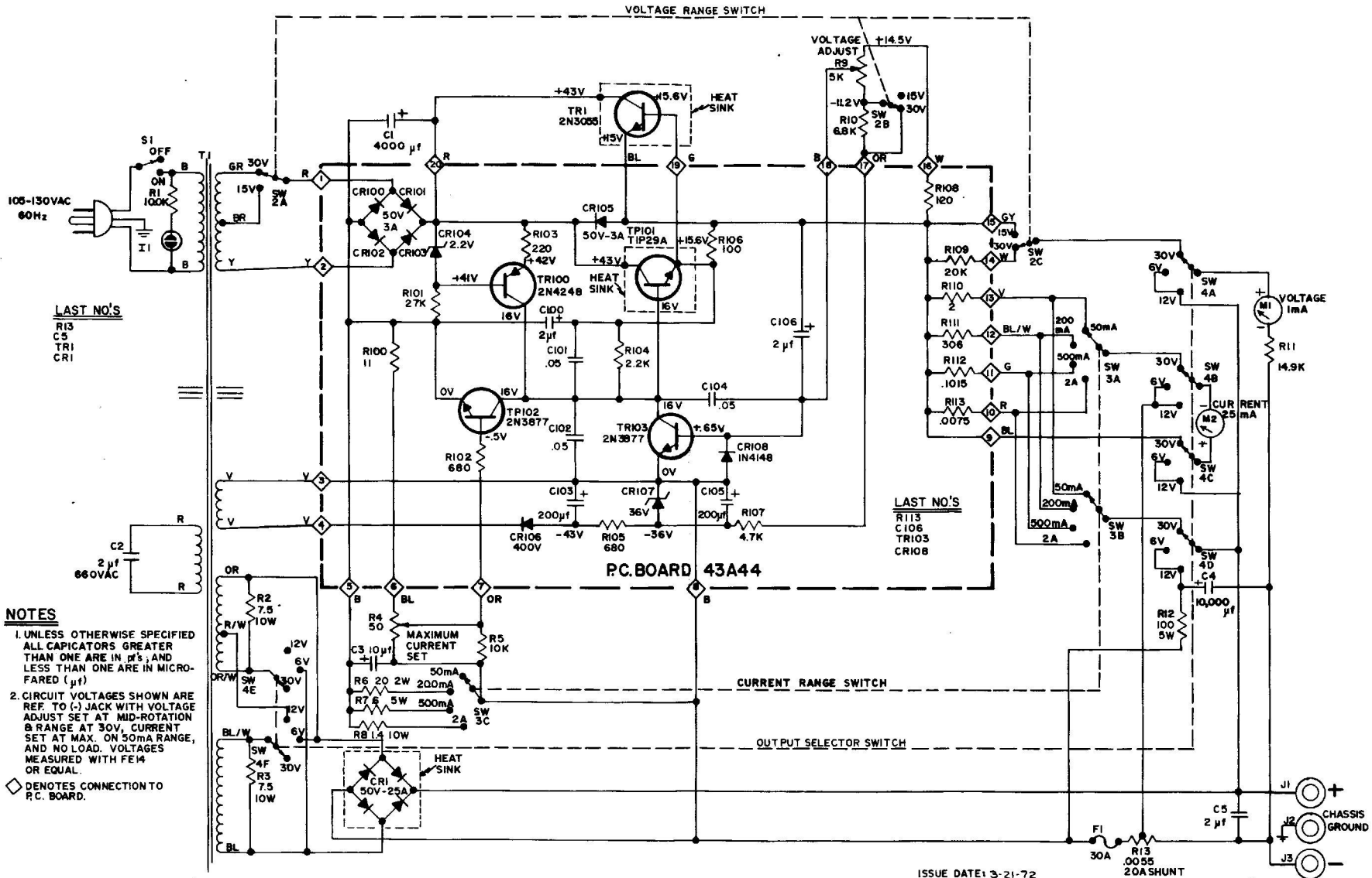
SCHEMATIC DIAGRAM UPS 164
