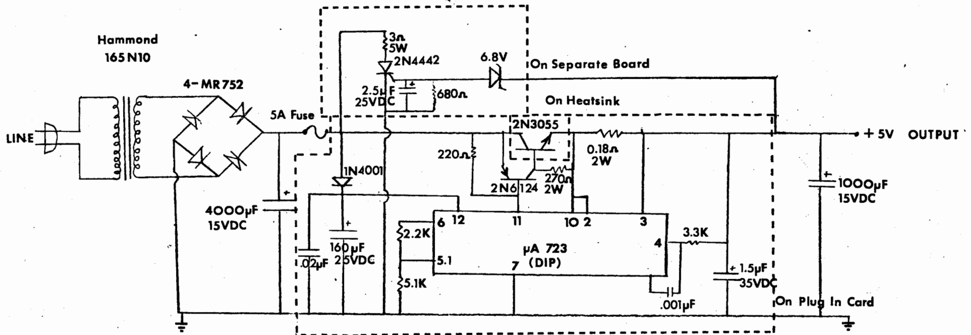
Regulated 5V 3A Power Supply In Killam Equipment
