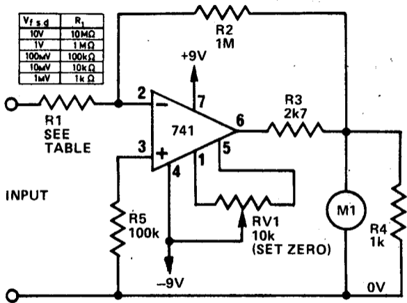
Fig. 27 High-performance d.c. voltmeter converter.
