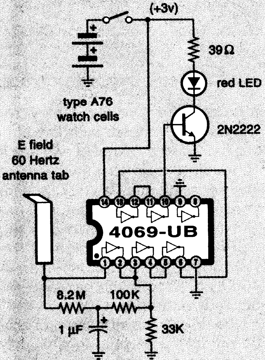
FIG. 4—A SIMPLIFIED SCHEMATIC of Radio Shack's 22 to 103 volt AC voltage sensor.
