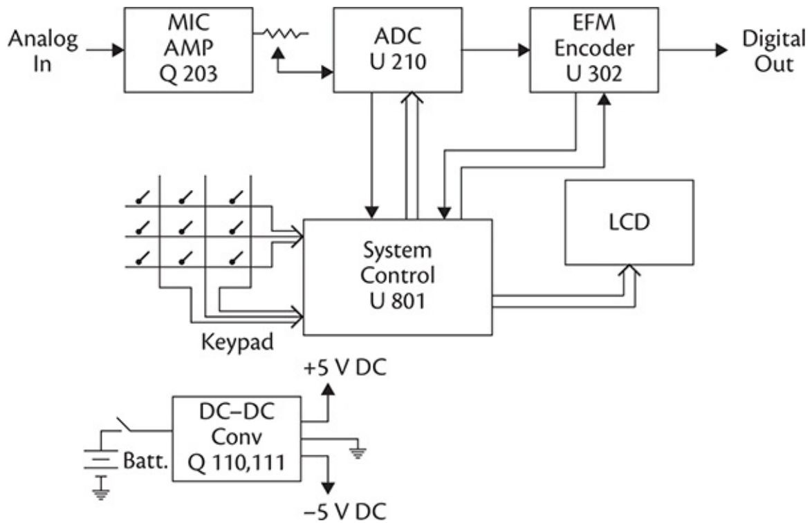
FIGURE 8-1 Block diagram.
