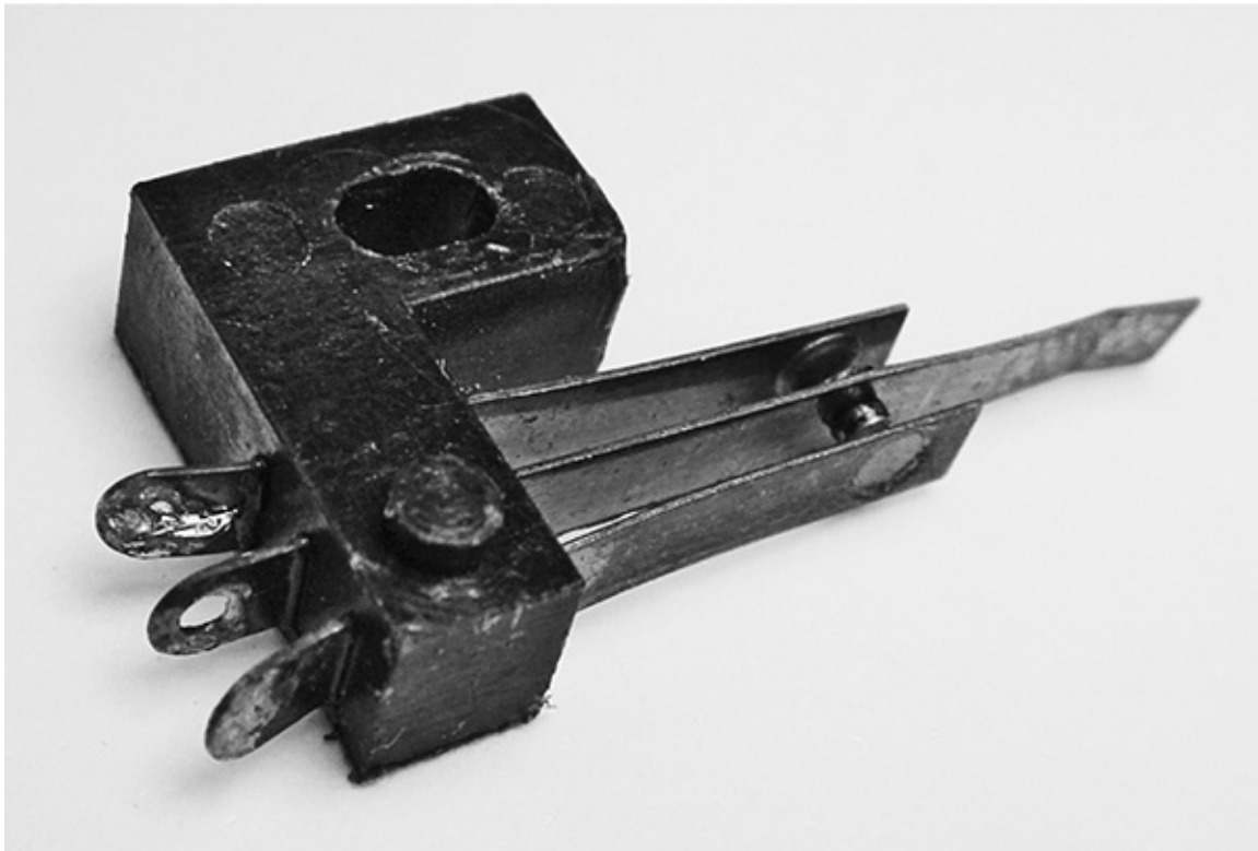
FIGURE 4-1 Leaf switch.
