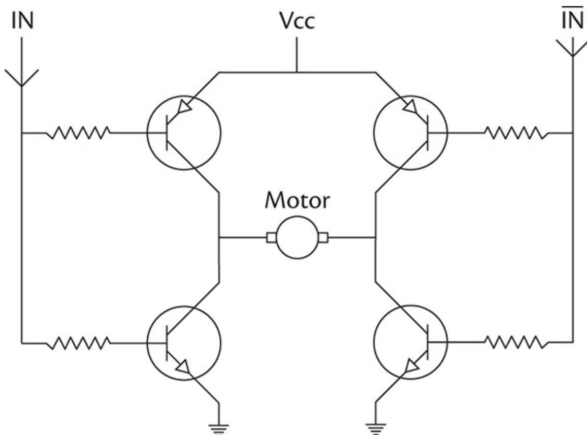
FIGURE 8-13 Typical H bridge.
