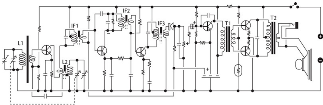
FIGURE 8-12 Classic superhetro AM radio schematic.
