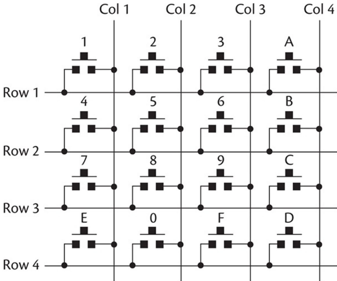
FIGURE 14-3 X-Y grid button diagram.
