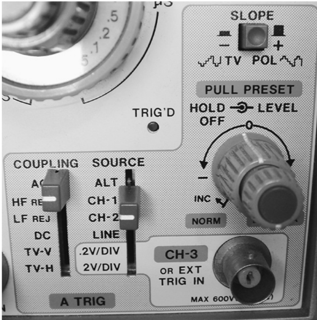
FIGURE 6-5 Trigger controls.
