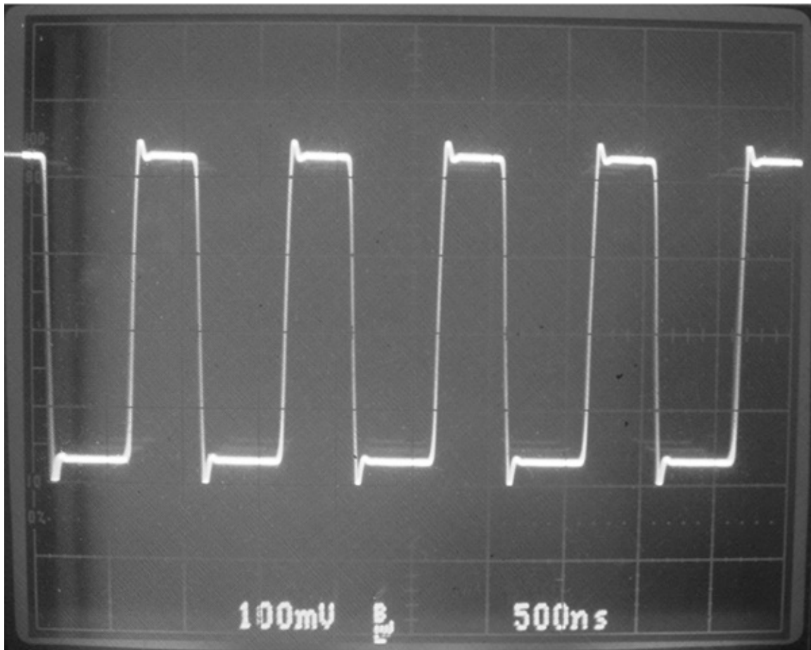
FIGURE 6-6 Probe overcompensation.
