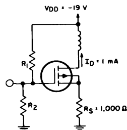
Fig. 8. Biasing circuit for an enhancement-type MOS transistor.
