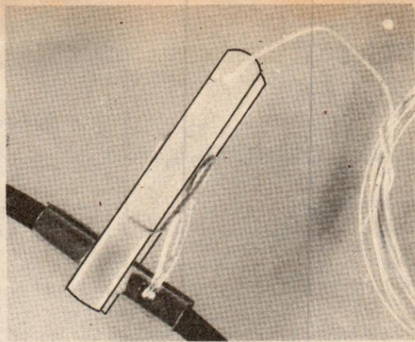
A simple pick-off can be made by gluing short lengths of split metal tube to a clothes peg.
