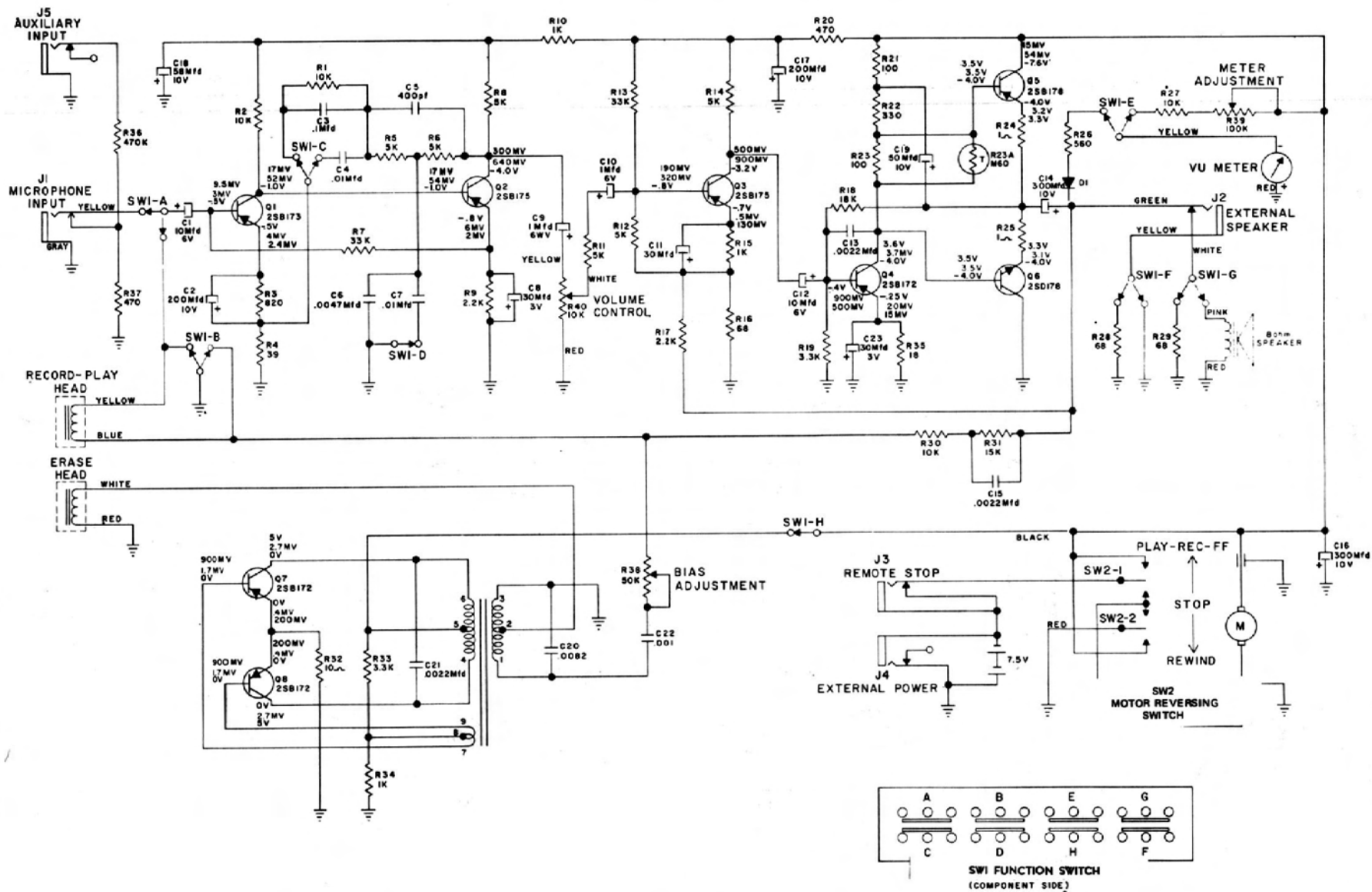
Fig. 5-57. Wollensak Model 4000 cordless cassette recorder. (Courtesy 3M Company)
