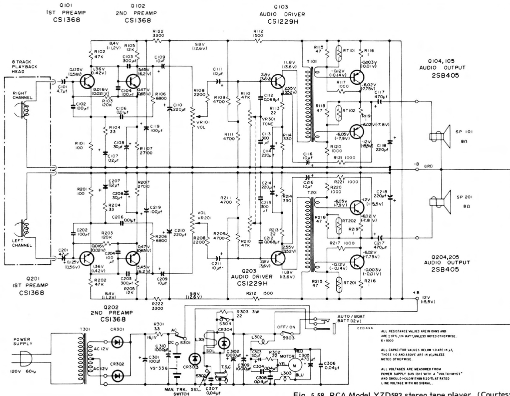
Fig. 5-58. RCA Model YZD593 stereo tape player. (Courtesy RCA)
