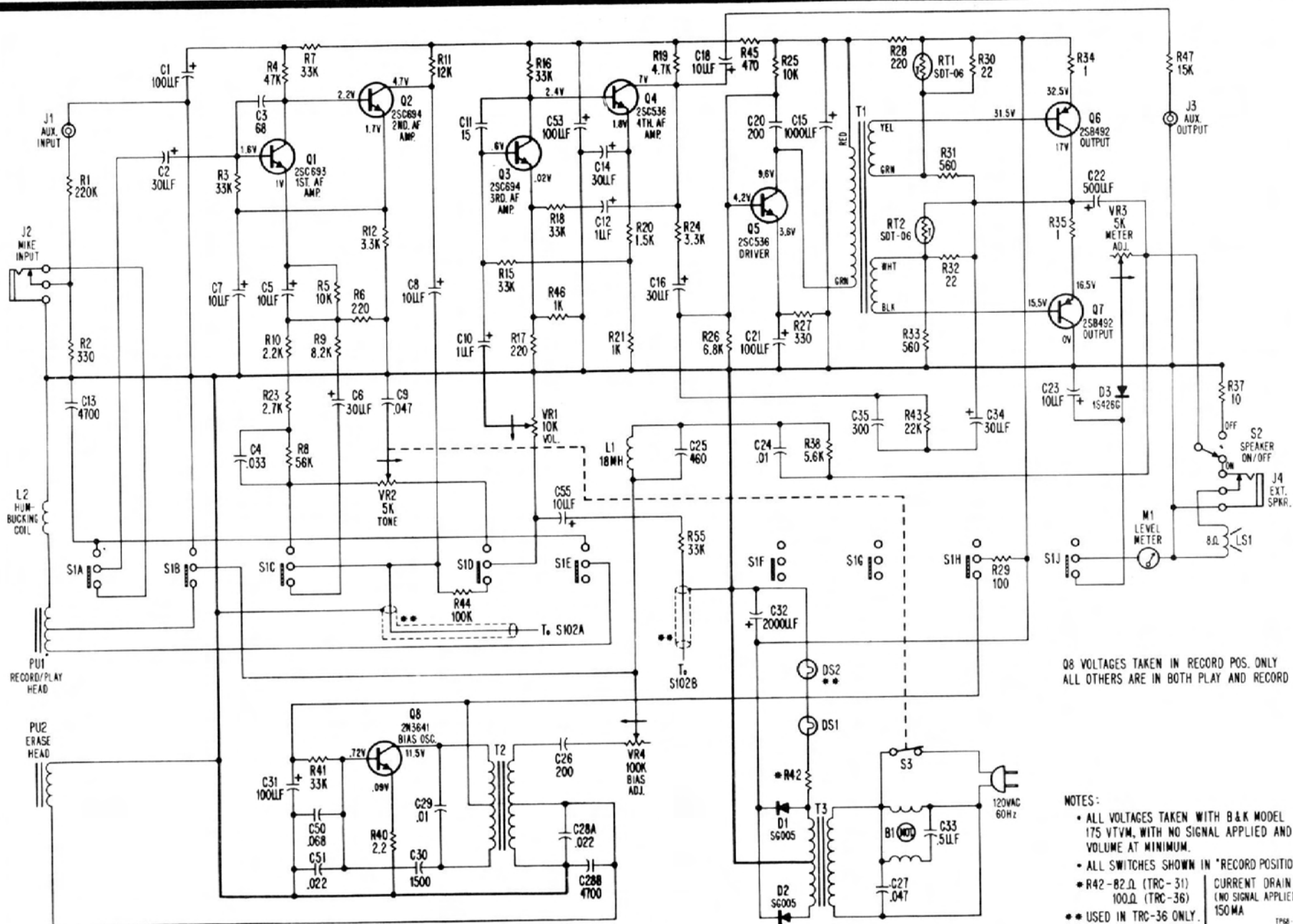
Fig. 5-53. Philco-Ford Model TRC-31, TRC-36 tape recorder. (Courtesy Philco-Ford Corp.)
