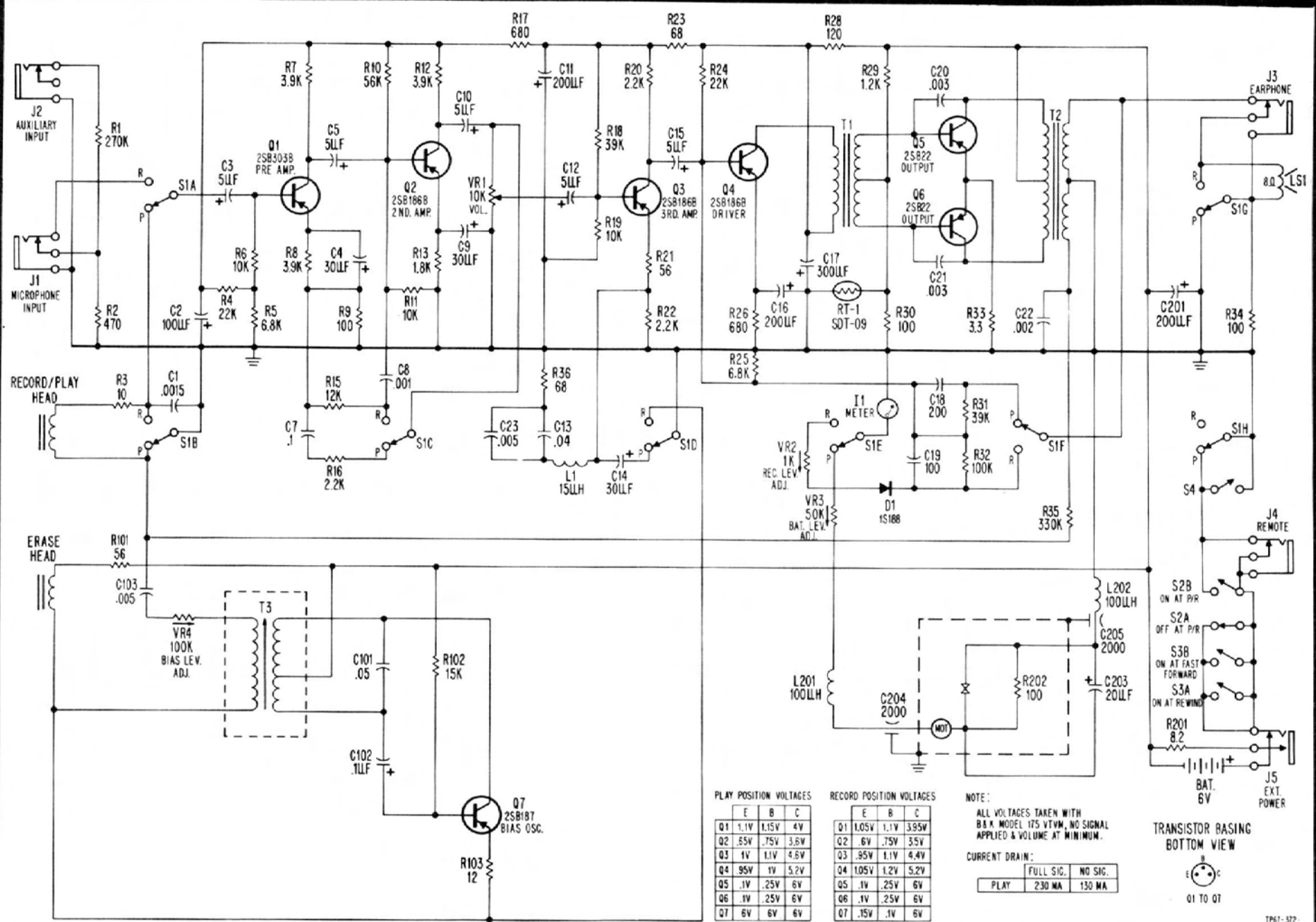
Fig. 5-52. Philco-Ford Model TRC-20 tape recorder. (Courtesy Philco-Ford Corp.)
