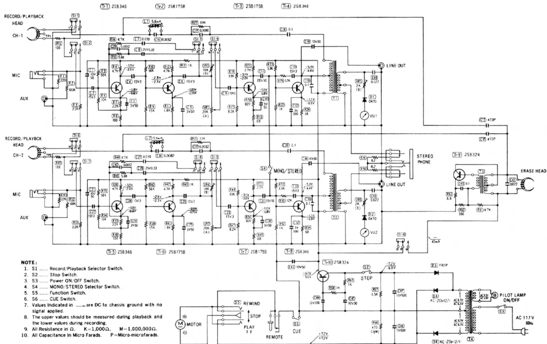
Fig. 5-51. Penncrest Model 6521 cartridge stereo tape recorder (made by Matsushita Electric Corp. of America). (Courtesy J. C Penney Co.)
