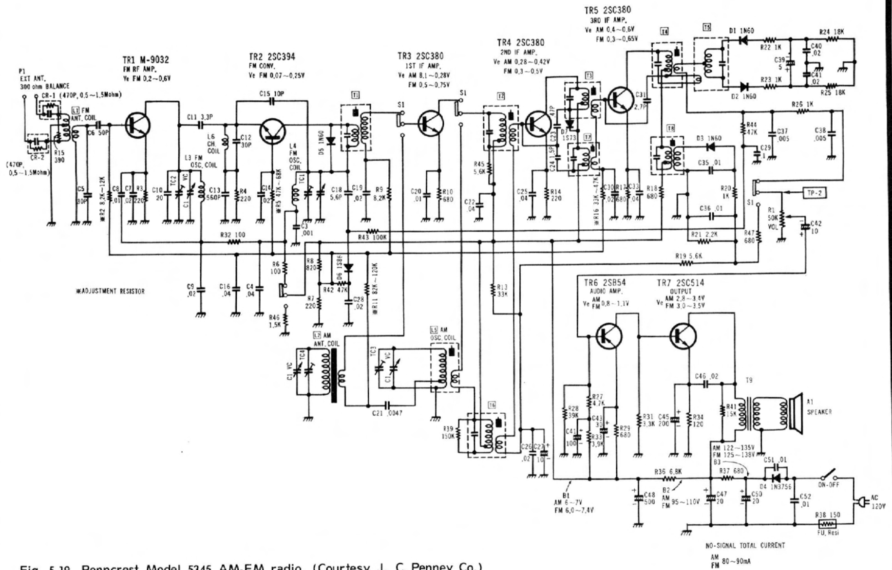
Fig. 5-19. Penncrest Model 5345 AM-FM radio. (Courtesy J. C. Penney Co.)
