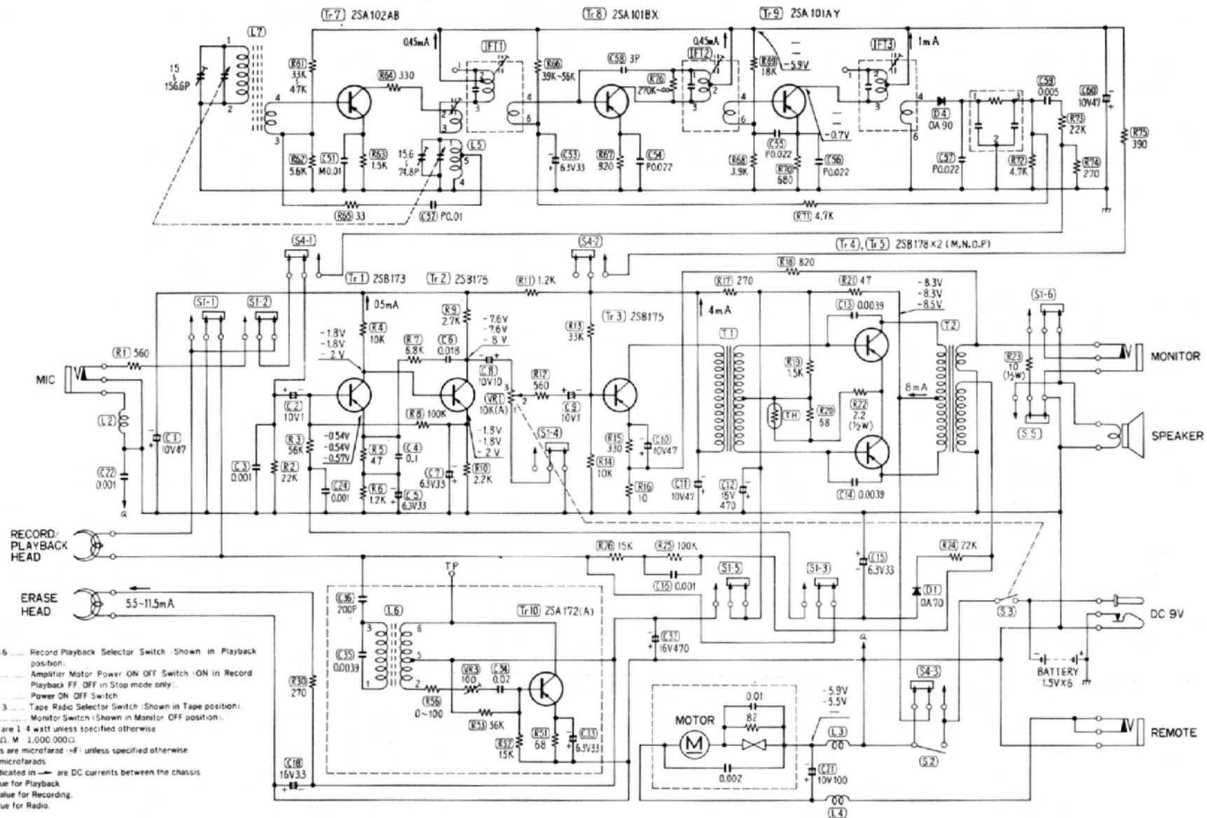
Fig. 5-50. Penncrest Model 3110 cassette tape recorder with AM radio (made by Matsushita Electric Corp. of America). (Courtesy J. C. Penney Co.)
