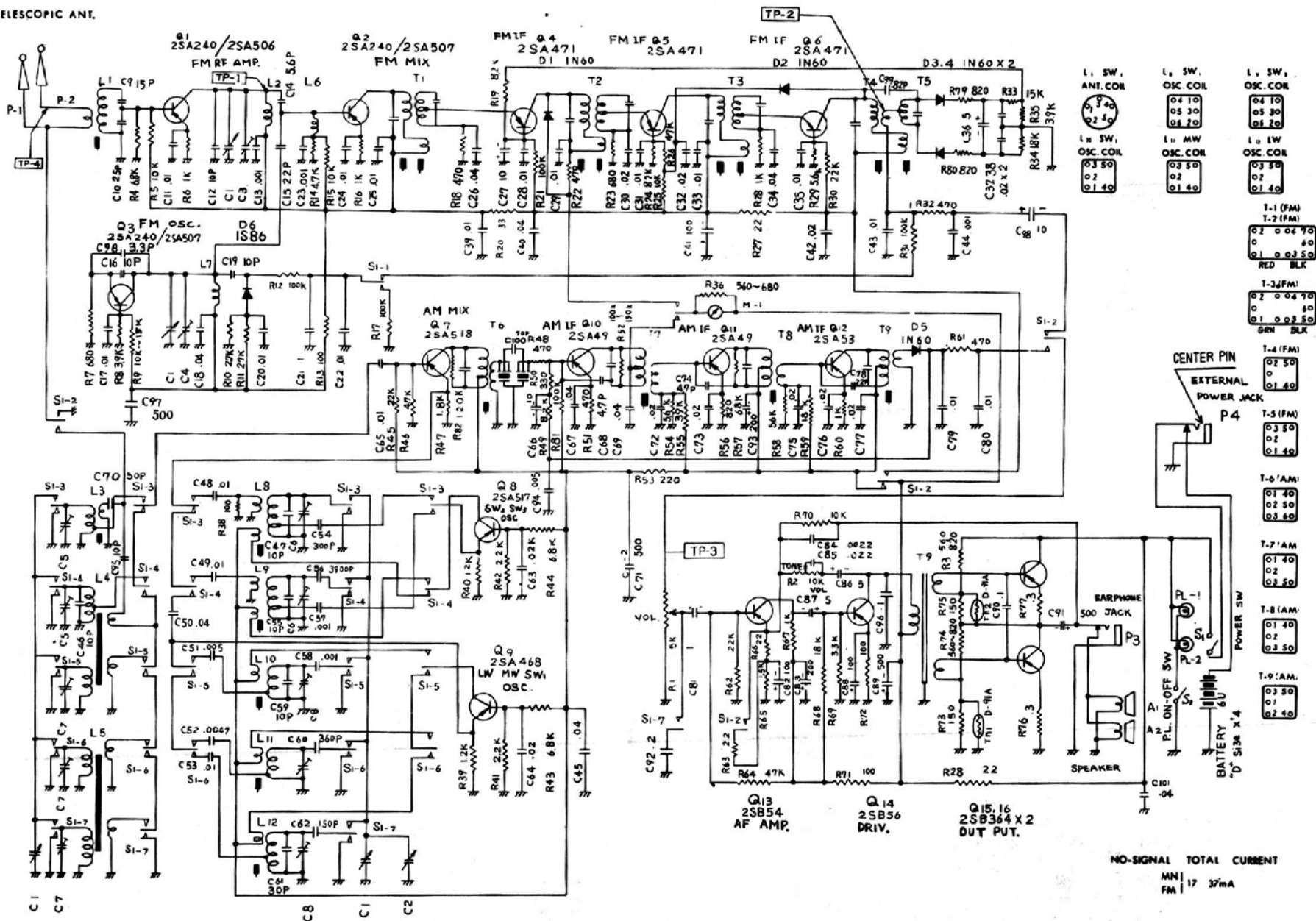
Fig. 5-18. Penncrest Model 1903A AM-FM portable radio. (Courtesy J. C. Penney Co.)
