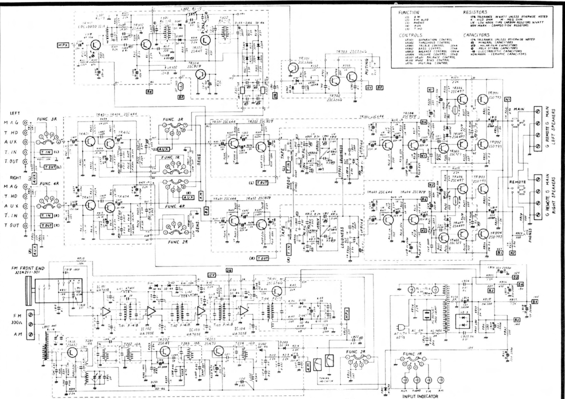
Fig. 5-29. Midland Model 19-560 AM-FM stereo receiver. (Courtesy Midland International Corp.)
