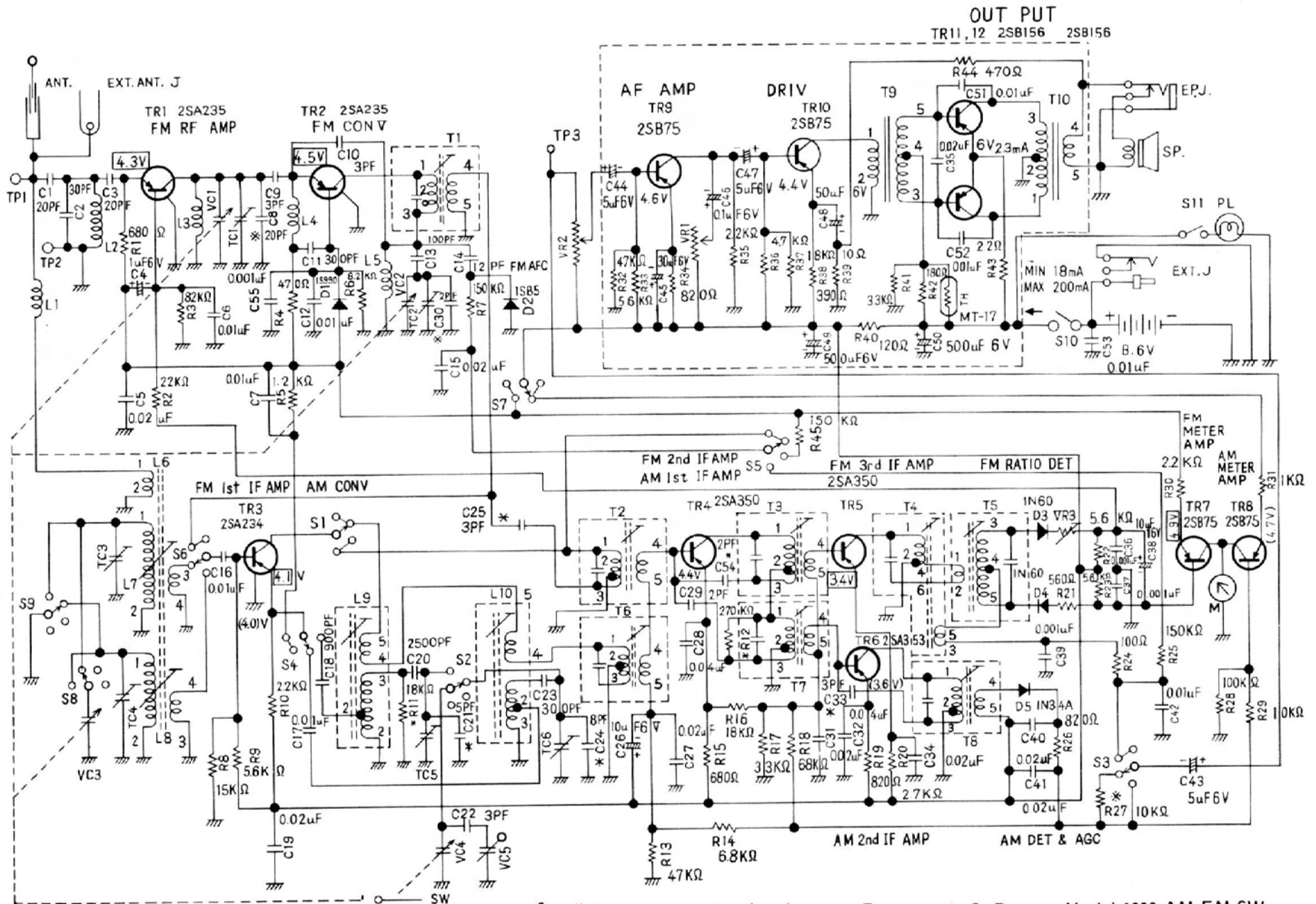
Fig. 5-37. J. C. Penney Model 1993 AM-FM-SW portable receiver. (Courtesy J. C. Penney Co.)
