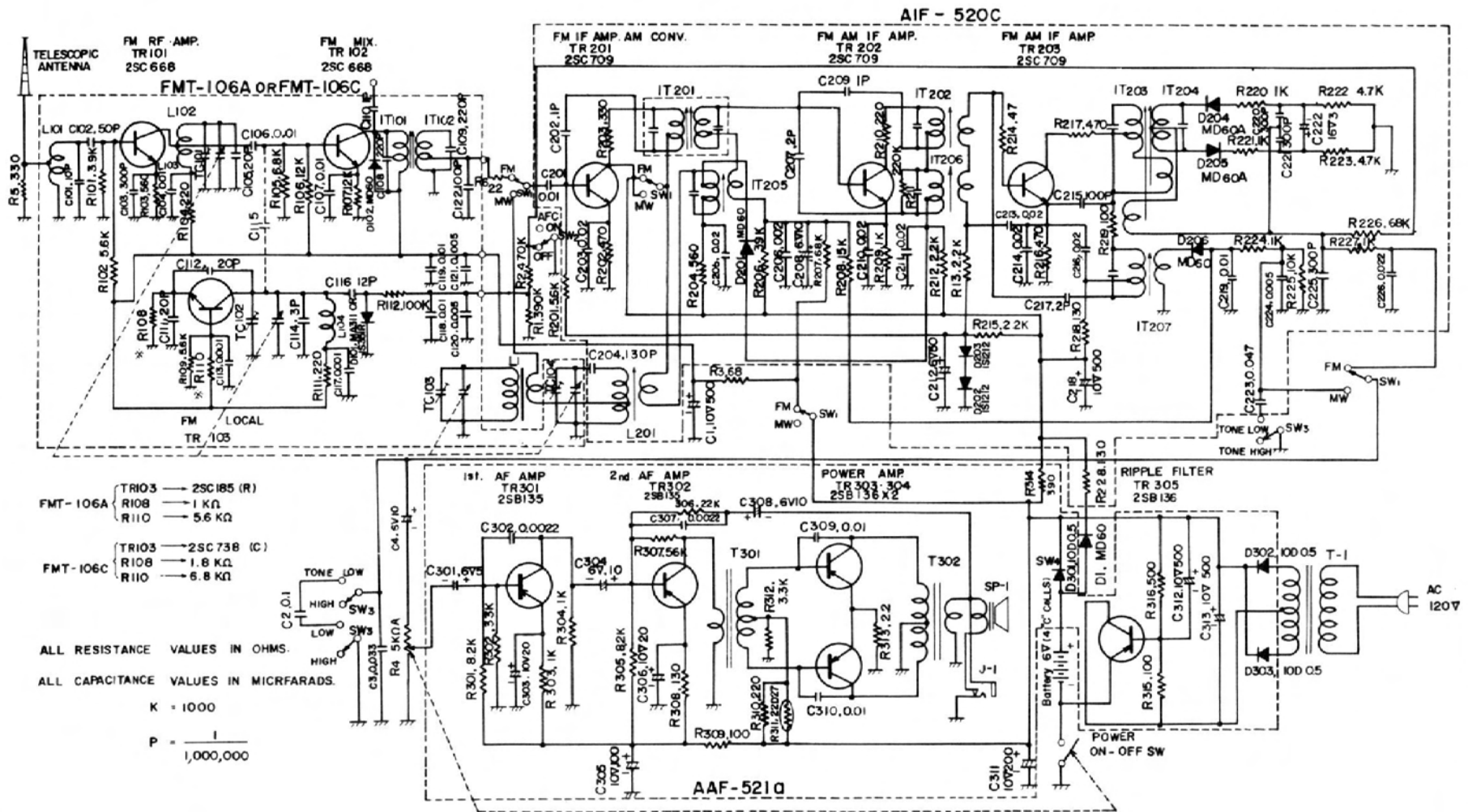
Fig. 5-12. Emerson Model 31P75 AM-FM, AC-DC radio. (Courtesy Emerson TV & Radio)
