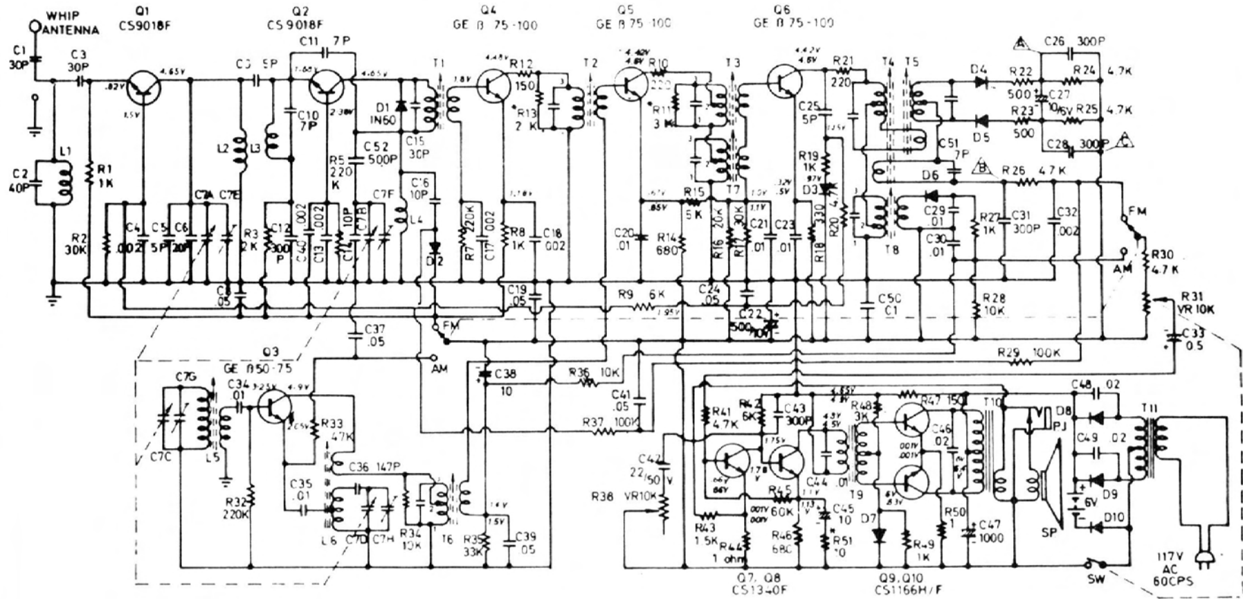
Fig. 5-13. Emerson Model 31P67 AM-FM radio. (Courtesy Emerson TV & Radio)
