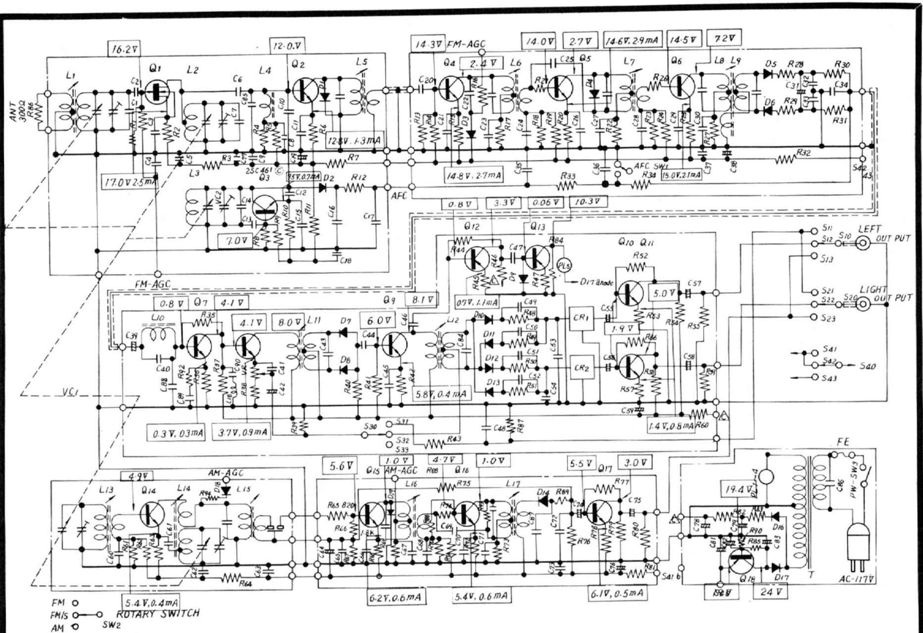
Fig. 5-27. Crown Model FM-500 AM-FM stereo tuner. (Courtesy Crown Radio Corp.)
