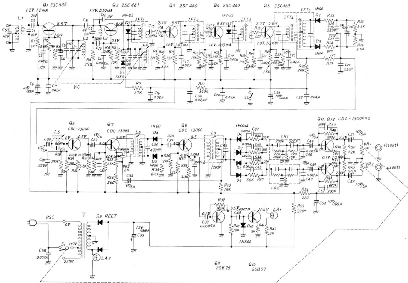
Fig. 5-26. Crown Model FM-300 FM stereo tuner. (Courtesy Crown Radio Corp.)
