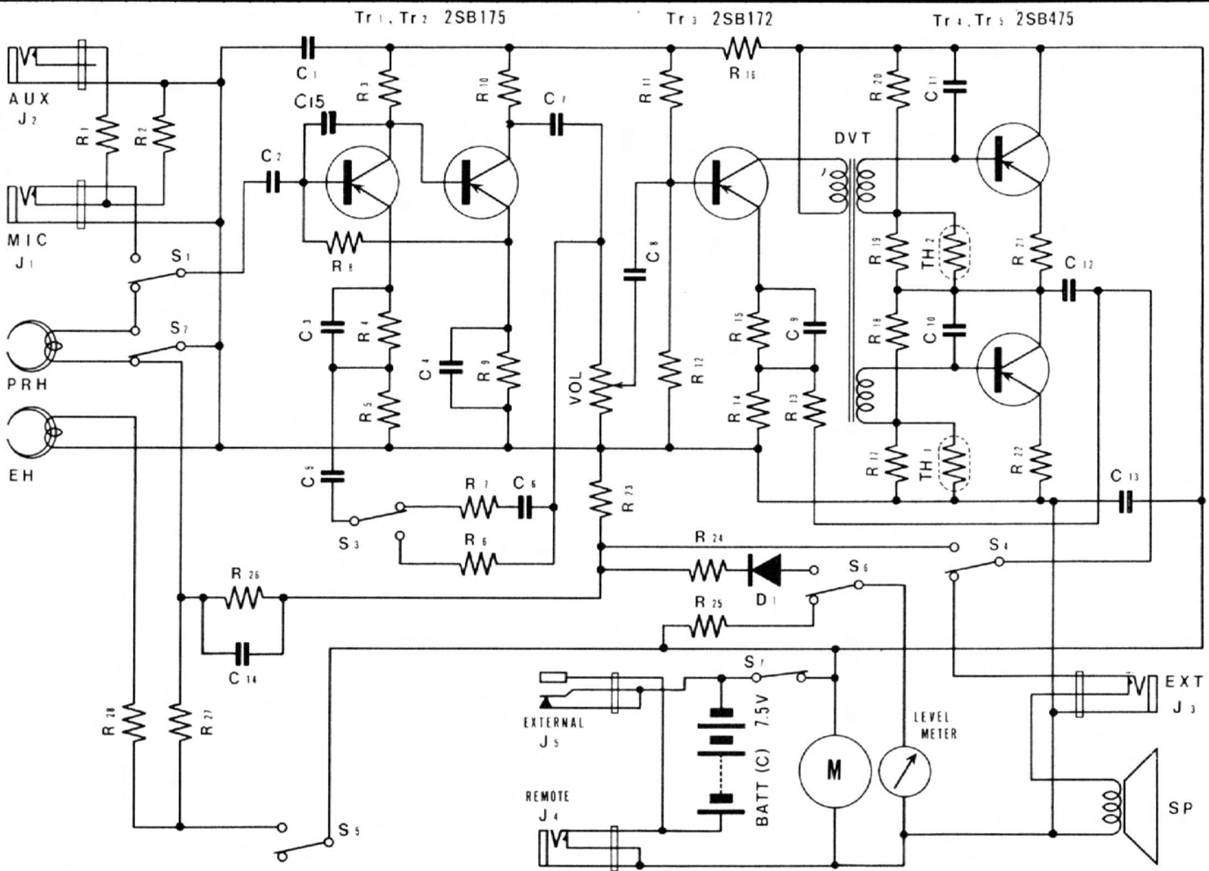
Fig. 2-10. Schematic diagram of the Channel Master Model 6305 cassette recorder. (Courtesy Channel Master)
