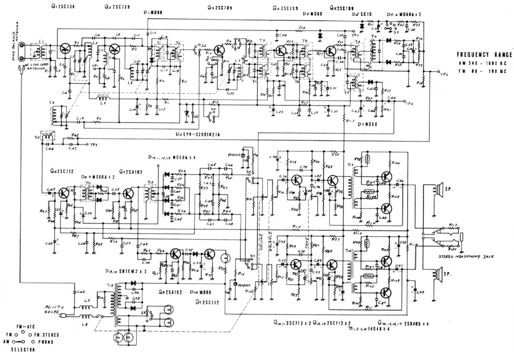
Fig. 5-10. Allied Model 2691 AM-FM radio. (Courtesy Allied Radio Corp.)
