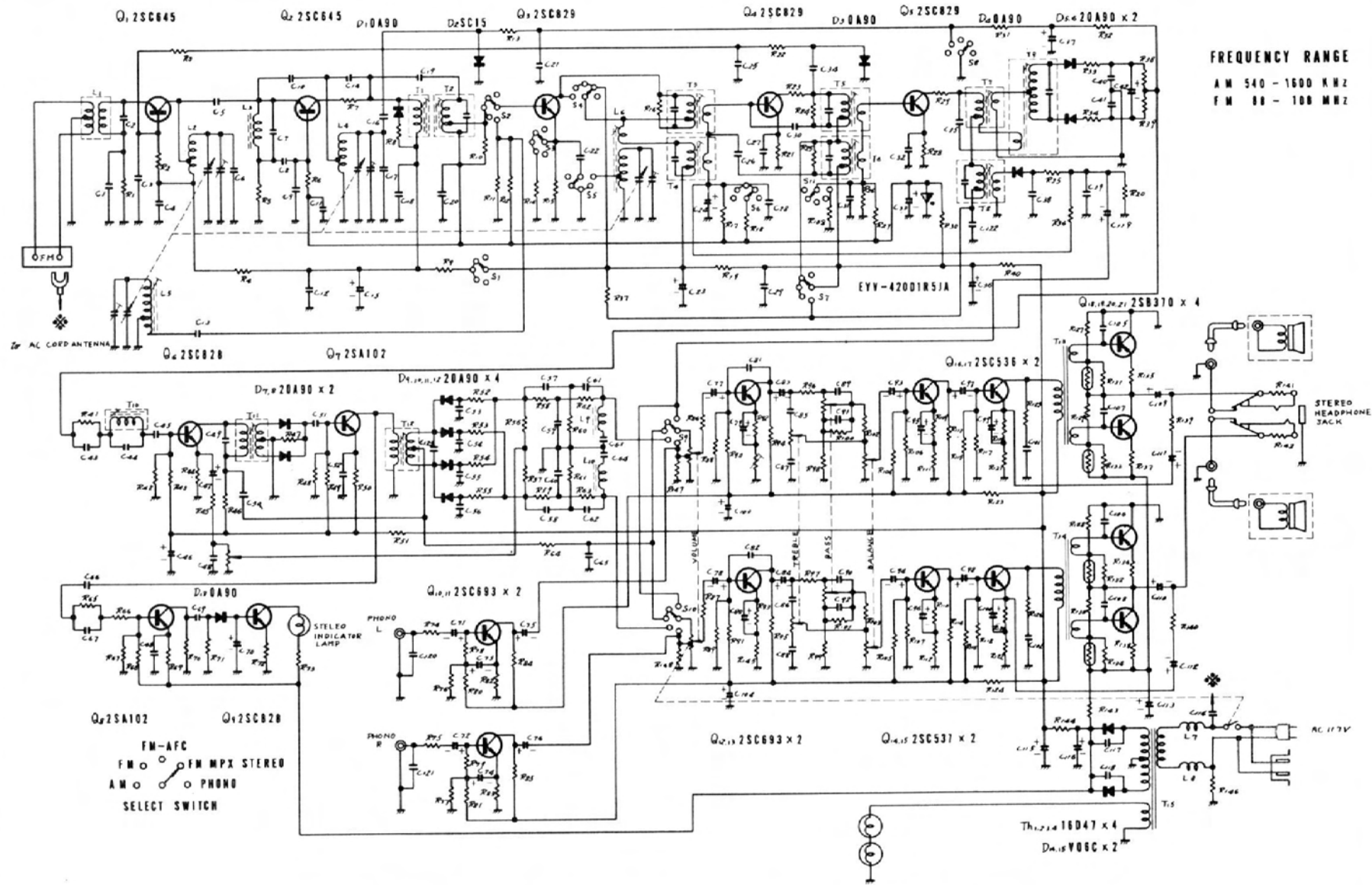
Fig. 5-11. Allied Model 2600 AM-FM radio. (Courtesy Allied Radio Corp.)
