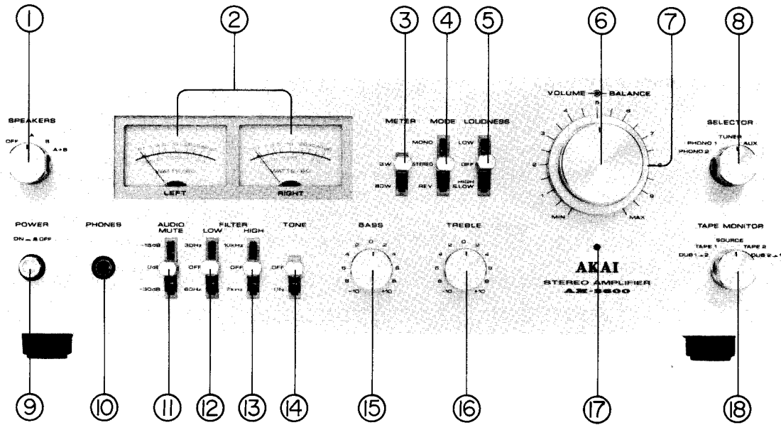
Fig. 1 Controls
