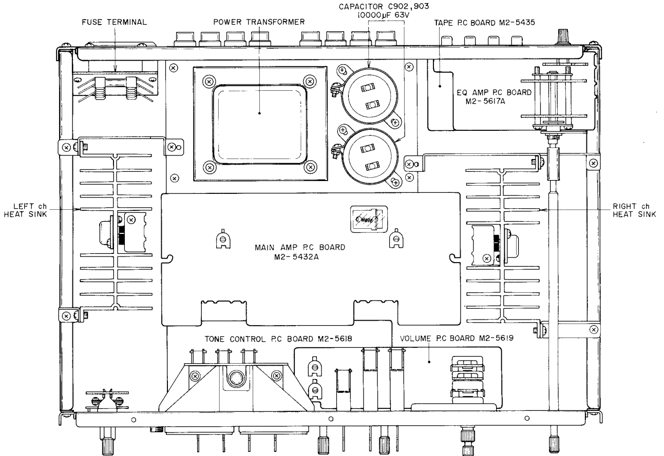
Fig. 2 Top View
