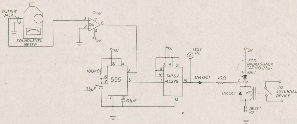
FIGURE 7 AN EXPERIMENTAL MOTION DETECTOR
