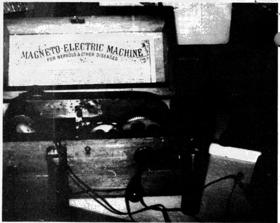
Fig. 6. In medical sine-wave generators a bobbin of wire is rotated in front of a permanent horse-shoe magnet. The design is almost identical with Clarke's 1830's original design and was still current around 1900.
