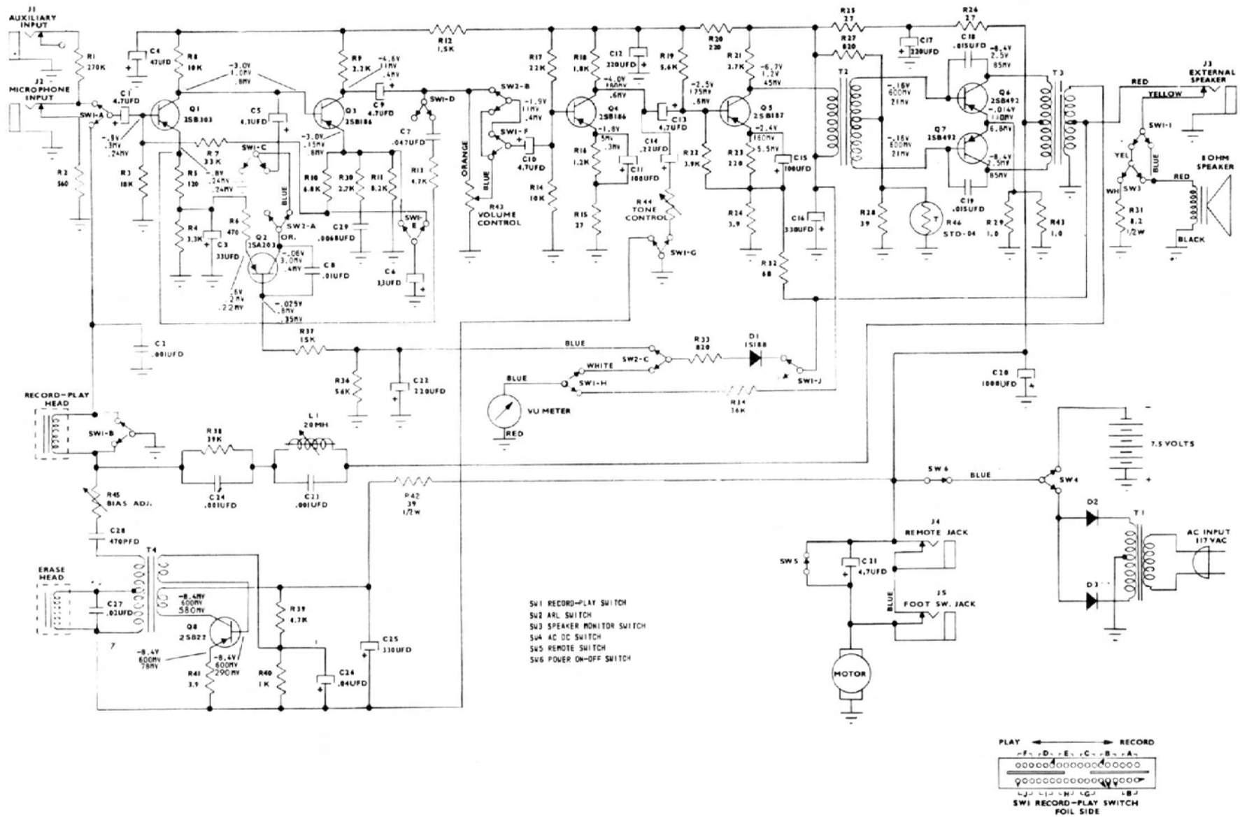
Fig. 5-72. Wollensak Model 4300 cassette tape recorder. (Courtesy 3M Company)
