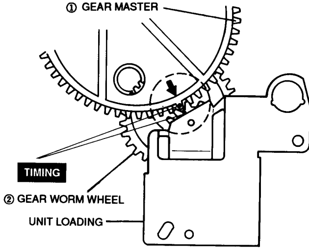
Fig. 48 Assembly of Gear Master
