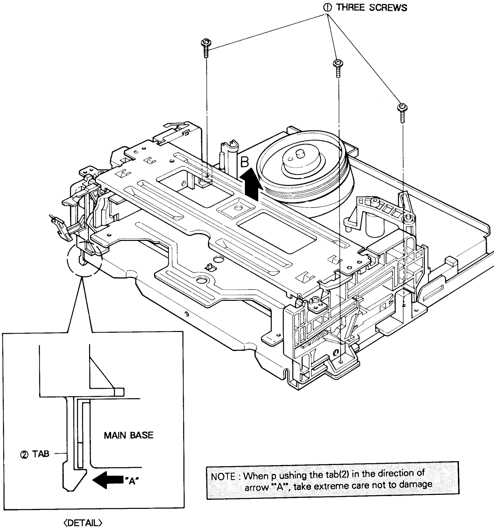
Fig. 12 Housing Ass'y Removal from Main Base
