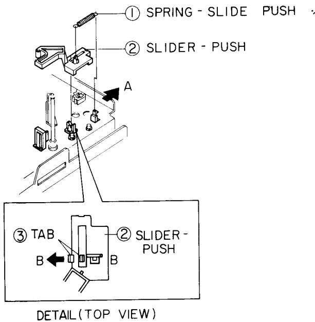
Fig. 60 Slide Push Removal
