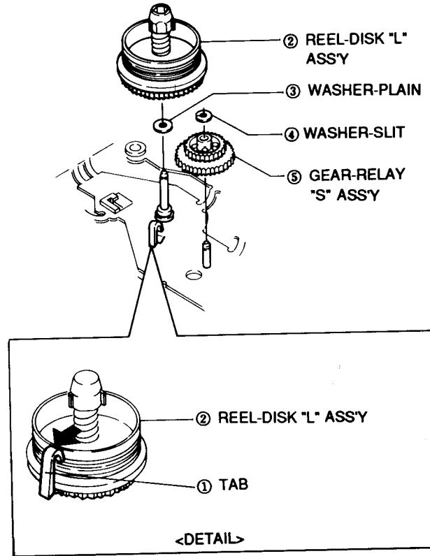
Fig. 31 Reel Disk "L" Ass'y & Gear Relay "S" Ass'y Removal
