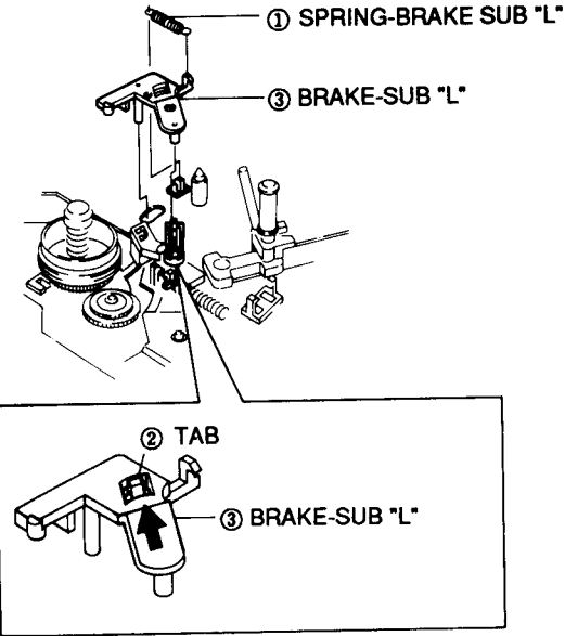
Fig. 29 Brake Sub "L" Removal
