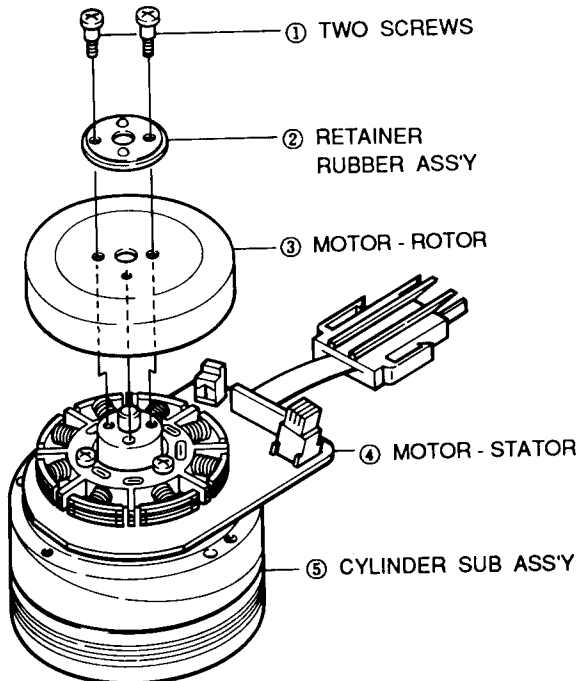
Fig. 23 Motor Rotor Removal
