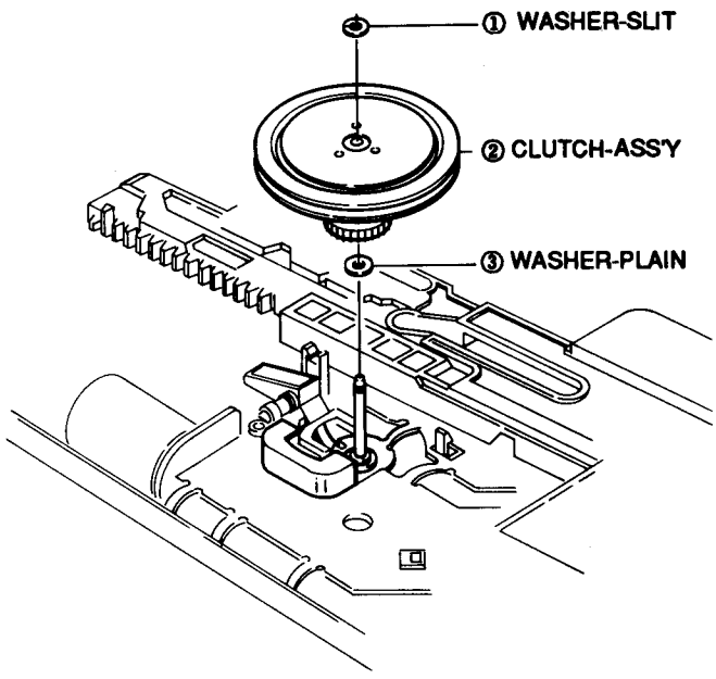
Fig. 46 Clutch Ass'y Removal
