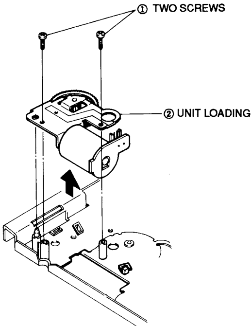
Fig. 49 Unit Loading Removal
