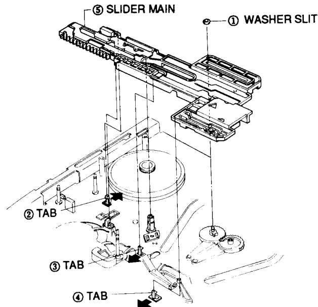
Fig. 52 Slide Main Removal
