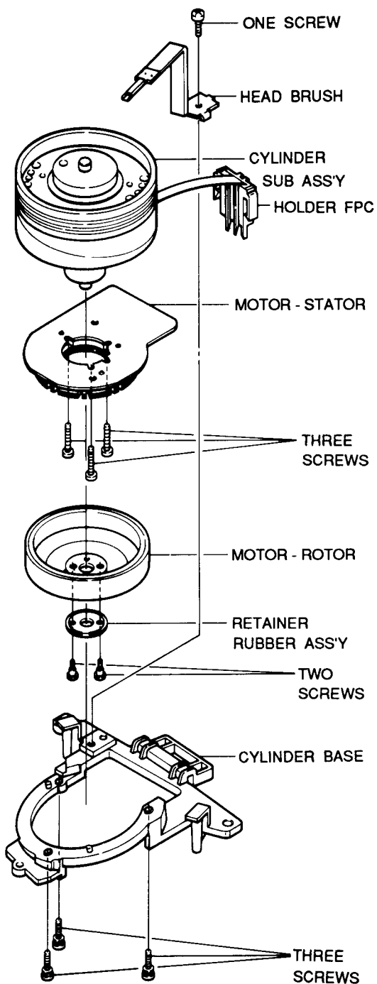
Fig. 18 Exploded View of Cylinder Ass'y
