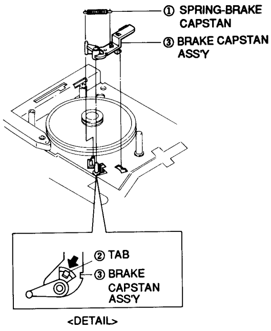
Fig. 44 Brake Capstan Ass'y Removal
