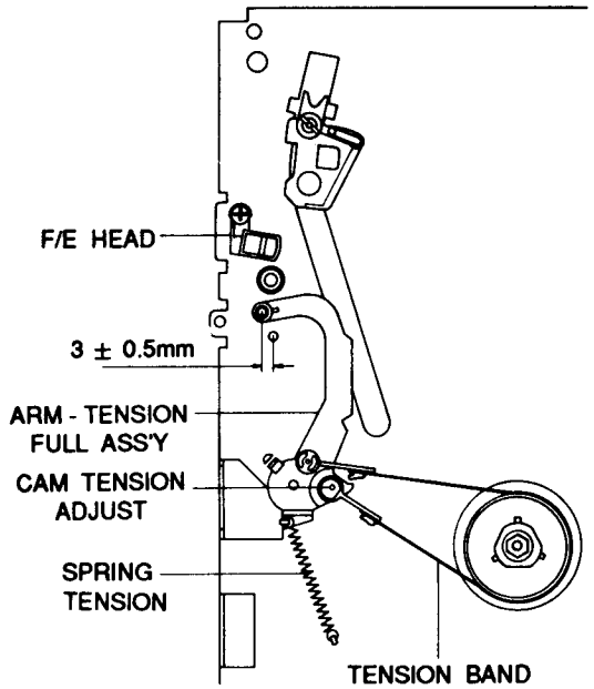
Fig. 16 Tension Pole and Back Tension Adjustment
