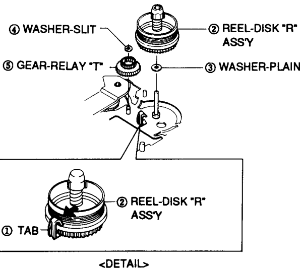
Fig. 33 Reel Disk "R" Ass'y & Gear Relay "T" Removal
