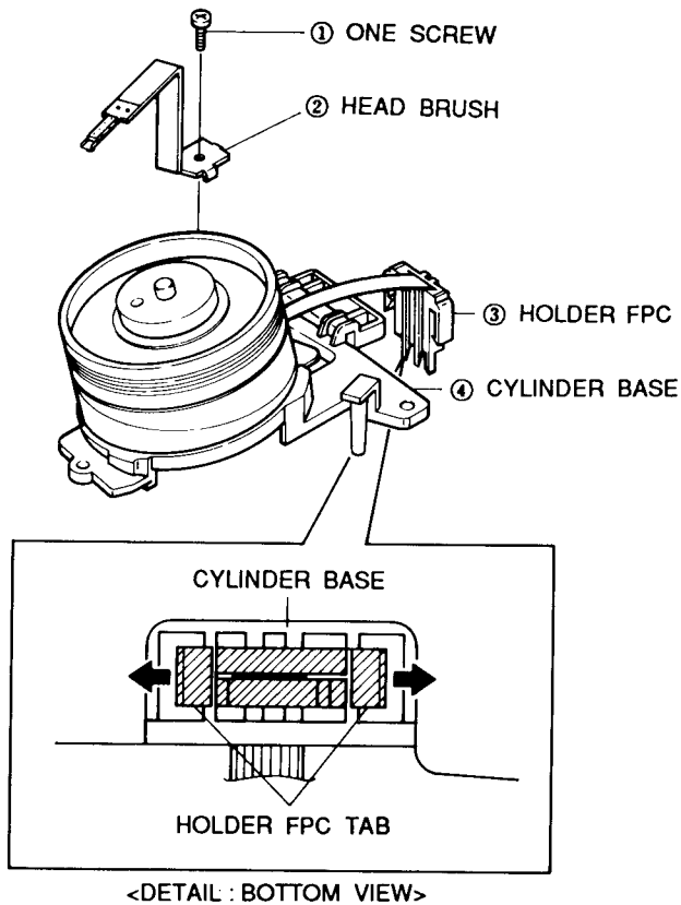
Fig. 21 Head Brush & Holder FPC Removal
