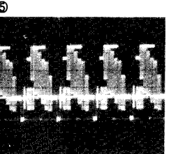
IC301-9 0.38Vp-p PB/REC
