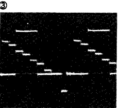
IC301-3 0.45Vp-p PB/REC
