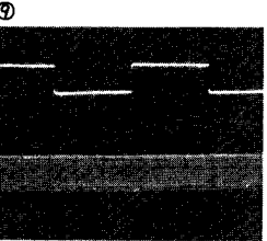
IC301-35 0.3Vp-p PB TP202 5.0Vp-p PB
