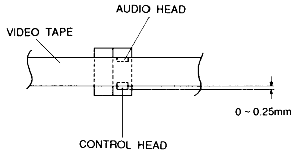
Fig. 5 A/C Head Height Adjustment
