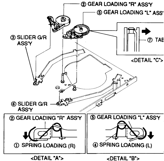
Fig. 57 Gear Loading "L", "R" Ass'y Removal
