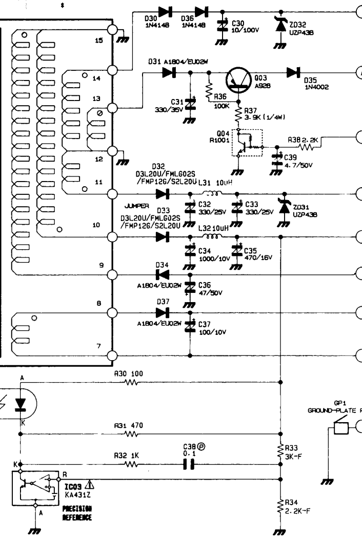
SMPS BLOCK
