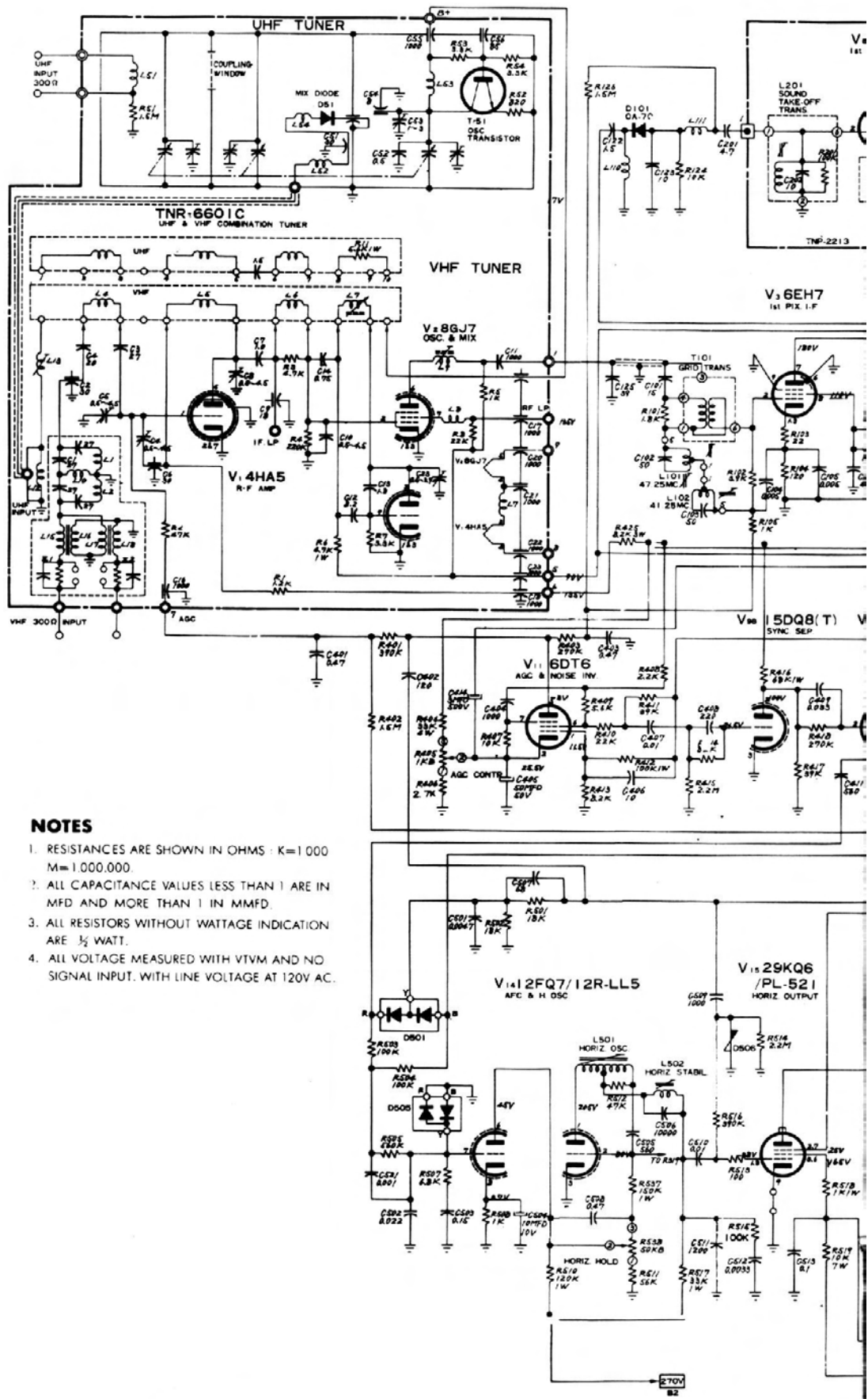
Panel K. Penncrest Model 2893 color TV (made by Matsushita Electric Corp. of America). (Courtesy J. C. Penney Co.)
