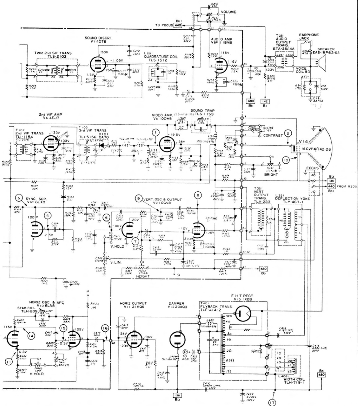
Fig. 5-69. Penncrest Model 2326 portable TV (made by Matsushita Electric Corp. of America). (Courtesy J. C. Penney Co.)
