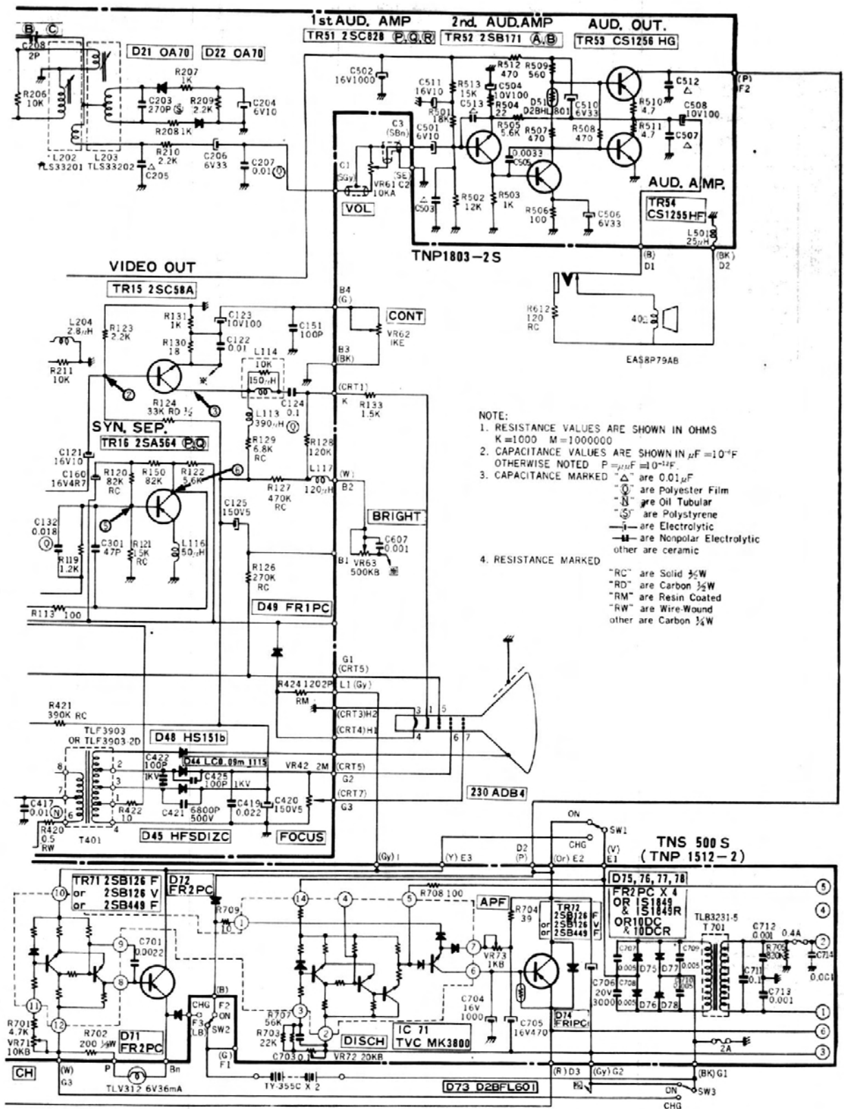
Fig. 5-64. Panasonic Model TR-449B AC-DC portable TV. (Courtesy Matsushita Electric Corp. of America)
