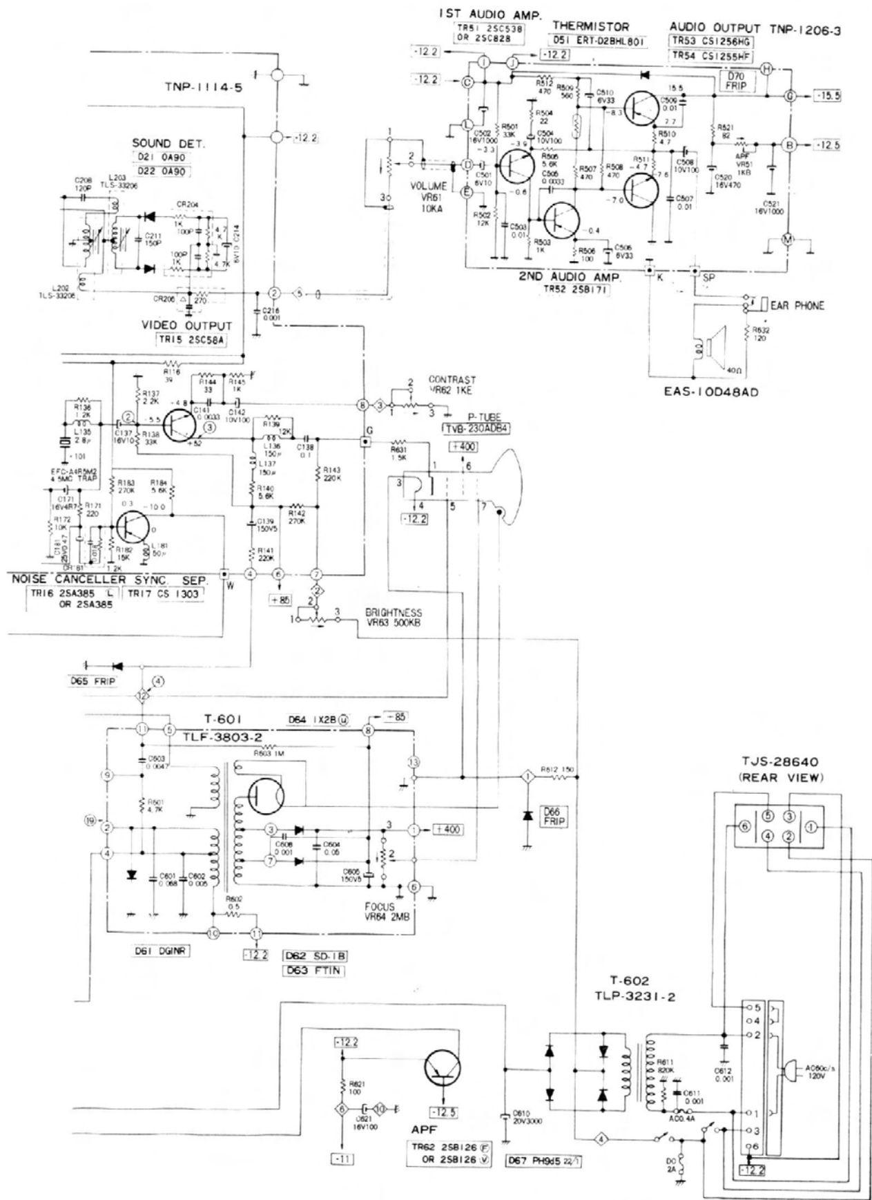
Fig. 5-62. Panasonic Model TR-329B AC-DC portable TV. (Courtesy Matsushita Electric Corp. of America)
