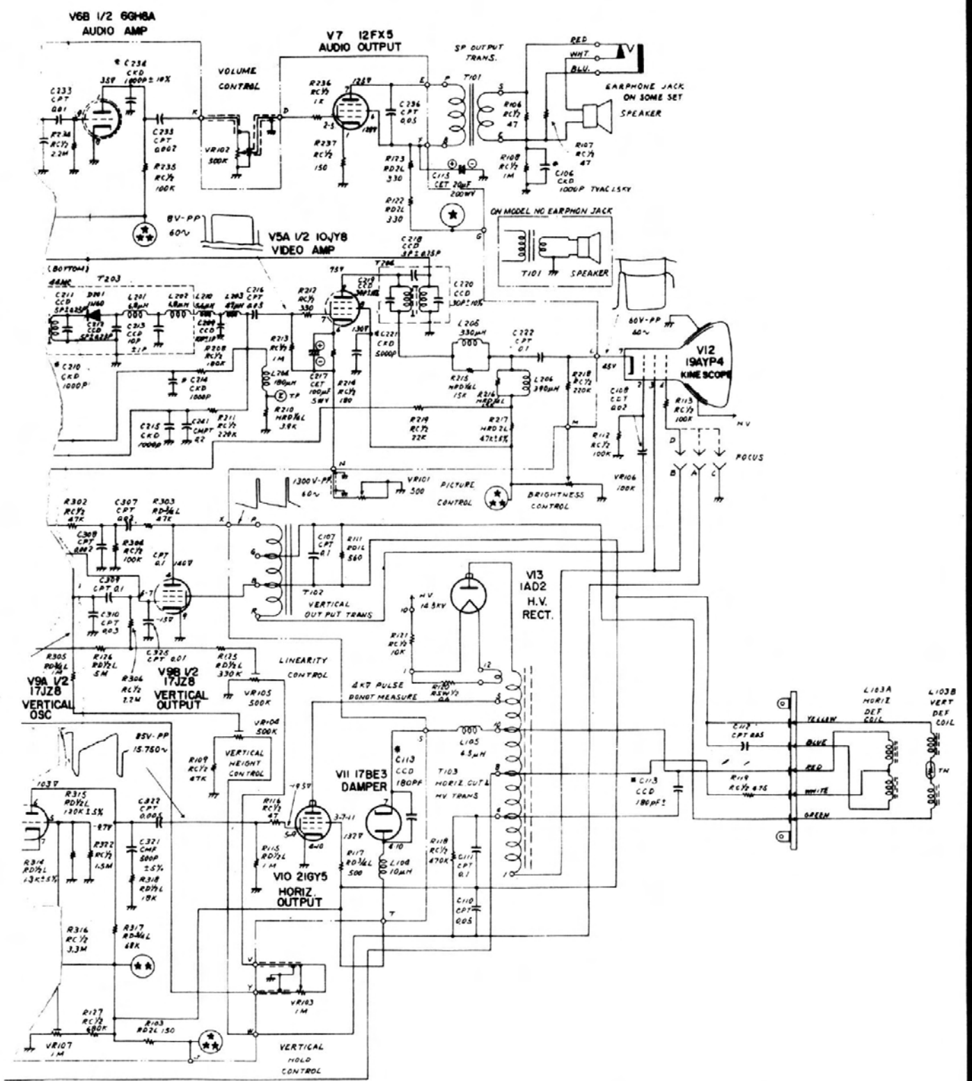
Fig. 5-71. Olympic Model 9P44, 45, 54 TV. (Courtesy Olympic Division Lear Siegler, Inc.)
