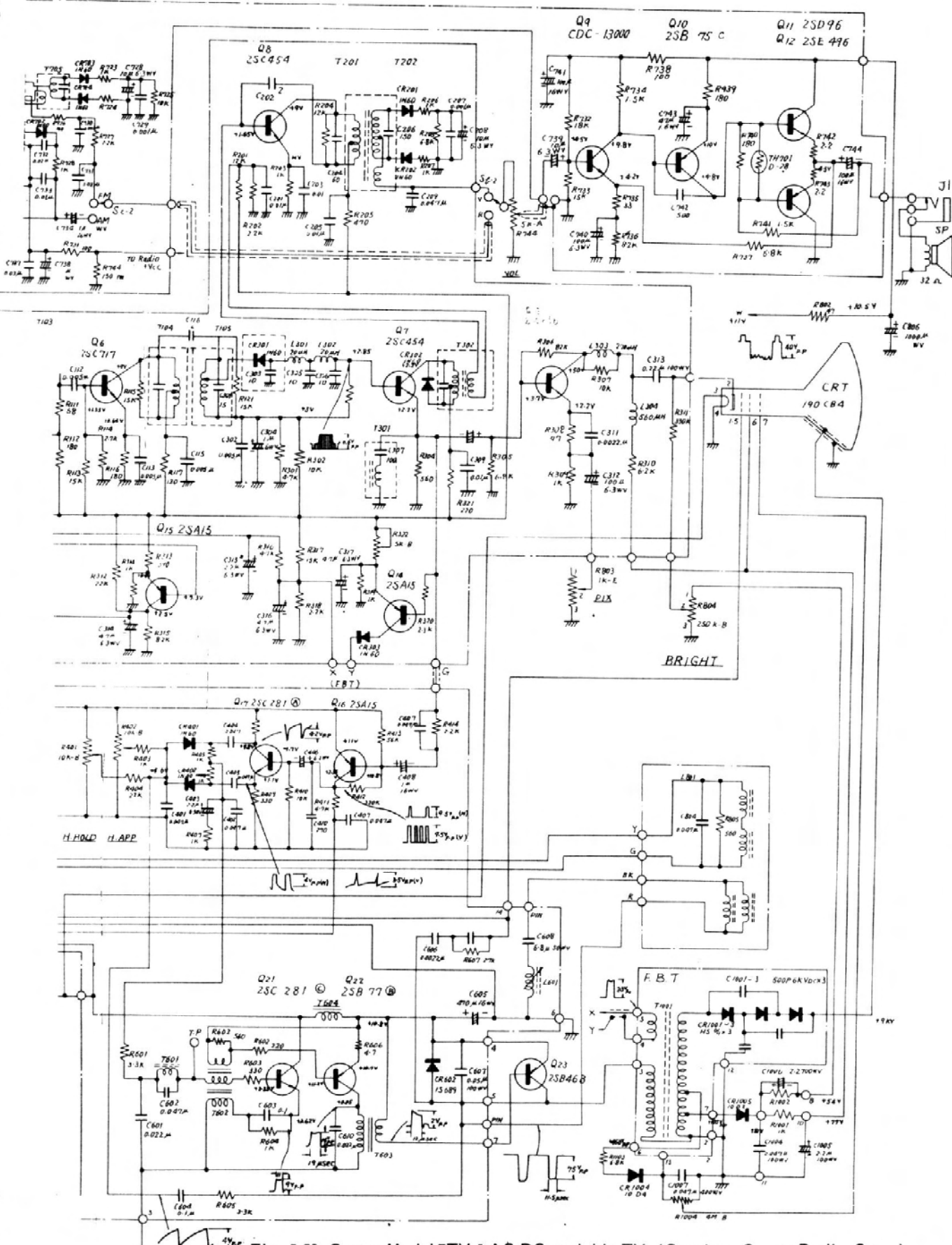
Fig. 5-59. Crown Model 7TV-1 AC-DC portable TV. (Courtesy Crown Radio Corp.)
