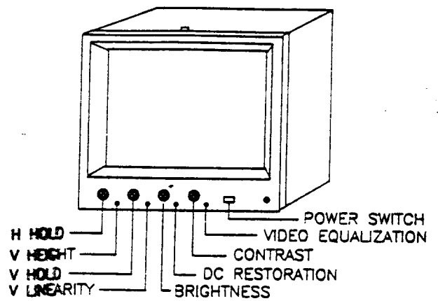
Figure 2 - Front Panel Controls
