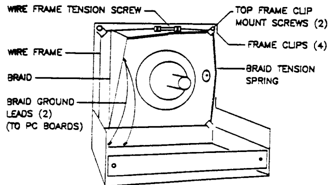
Figure 13 - CRT Removal
