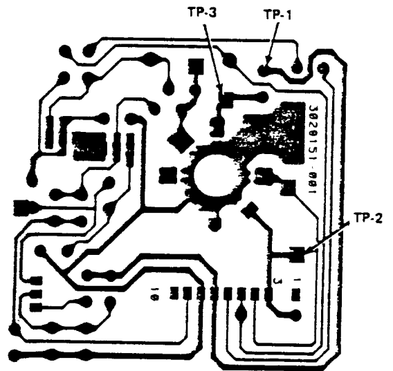
Figure 3 - Test Points
