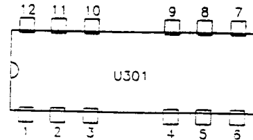
Figure 7 - IC U301 Pin Layouts
