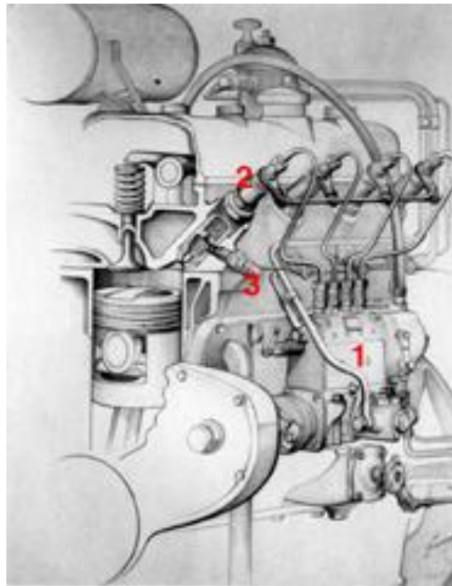
1. Pump 2. Injector 3. Glow plug
