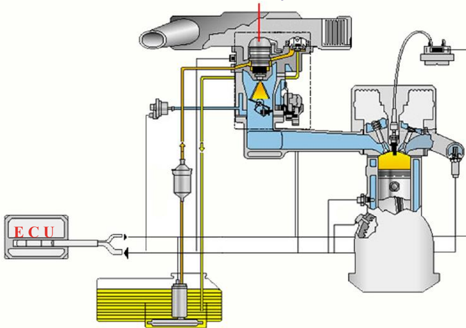
Mono injector
