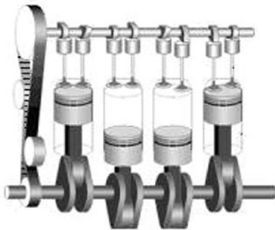
3. "OHC" engine
