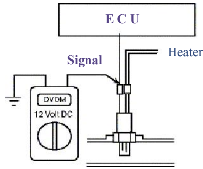
Sensor with three wires
