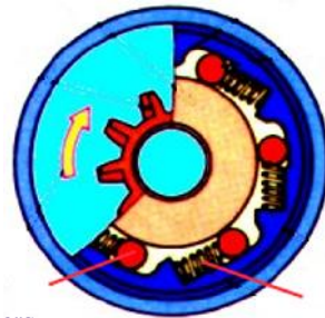
Rollers
