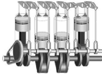
2. "OHV" engine
