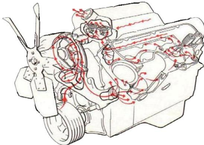
Engine coolant circulation
