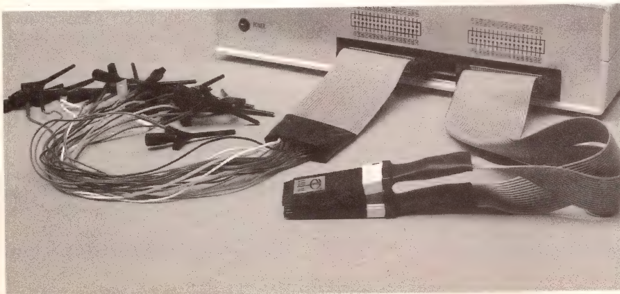
For general work, two different kinds of input probe are most useful: a set of individual EZ-HOOK leads like those at left, and a 16-pin DIL IC clip like that at right.
