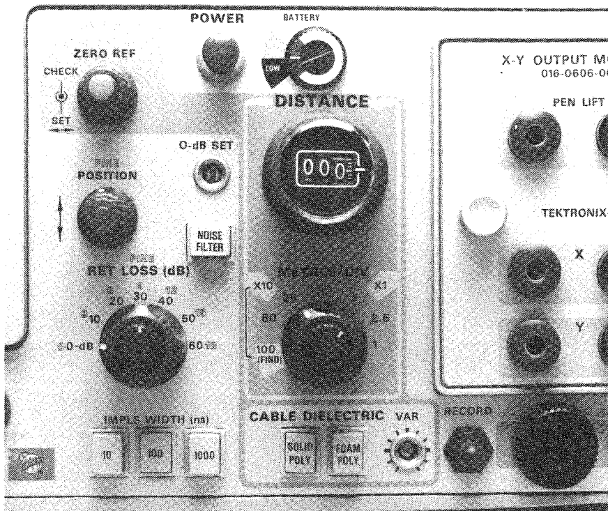
FIG. 6—FRONT PANEL OF TEKTRONIX' MODEL 1503 TDR has controls that calibrate the CRT for direct distance display.
