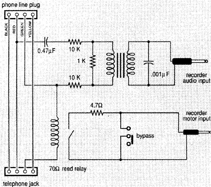
FIG. 3—AN AUDIO-ACCESS ARRANGEMENT can record both sides of a telephone conversation, but is only legal for use under certain circumstances.
