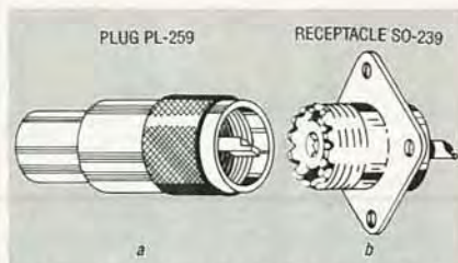
FIG. 7—A STANDARD PLUG AND RECEPTACLE used to mate two coaxial cable sections; (a) is a PL-259 plug and (b) is an SO-239 receptacle.
