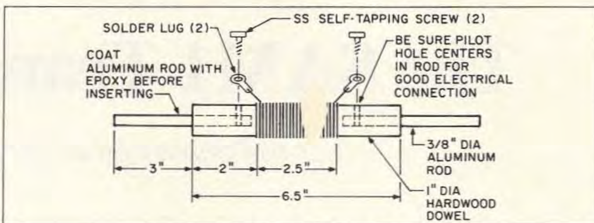
Figure 5. Loading coil assembly.
