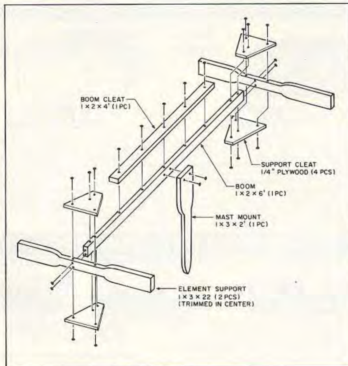
Figure 3. Boom assembly.
