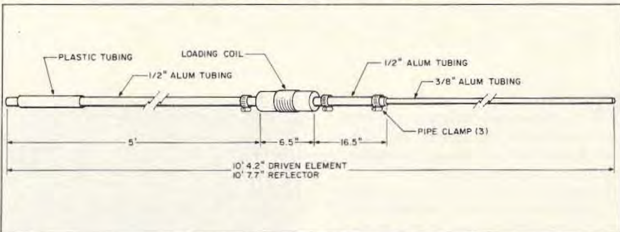
Figure 6. Element assembly (times four).
