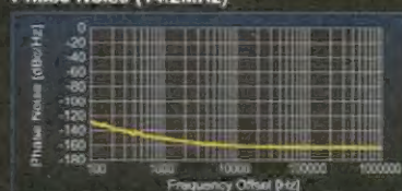
1st Local OSC Phase Noise (14.2MHz)
