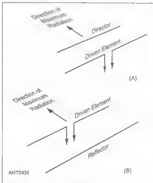
Figure 7.8 — Two-element Yagi antennas using a single parasitic element. At A the parasitic element acts as a director, and at B as a reflector. The arrows show the direction of maximum radiation.
