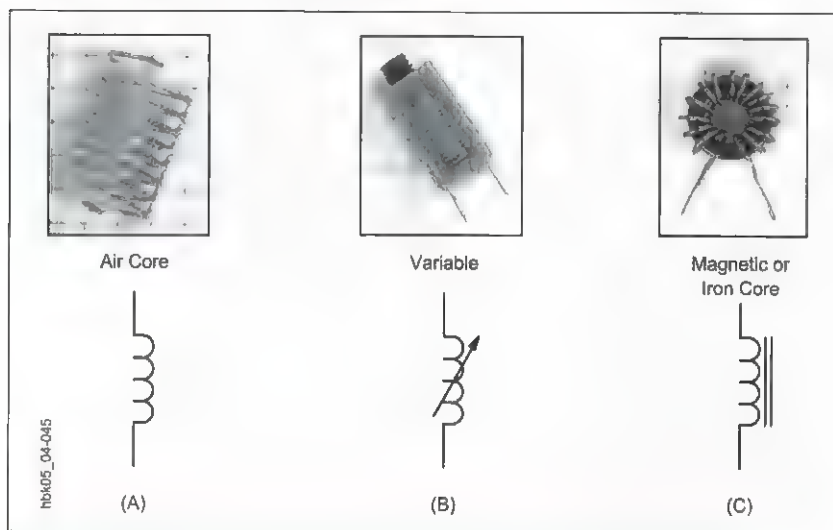
Figure 4.6 — Photos and schematic symbols for common inductors.
