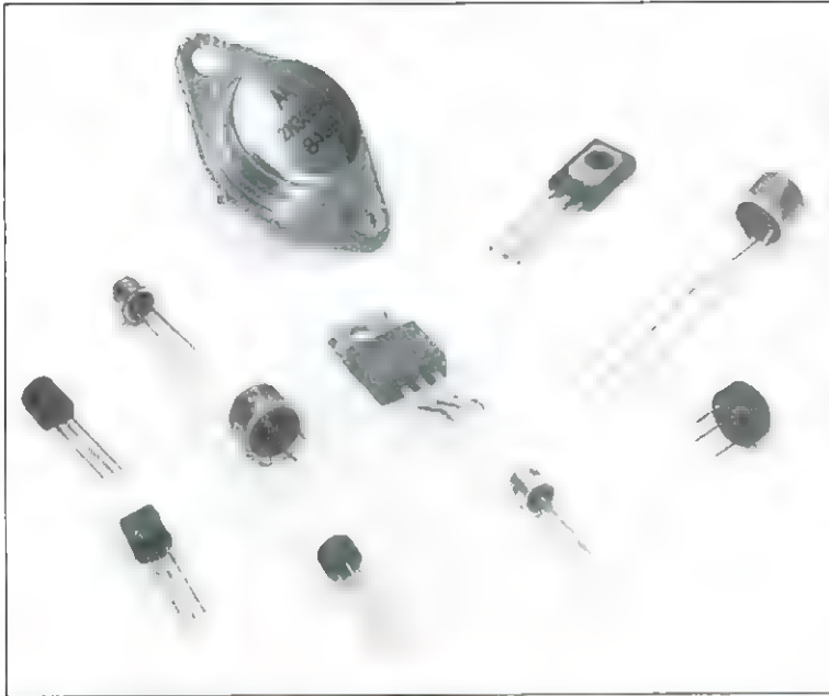
Figure 4.21 — Transistors come in a variety of package styles. The smaller packages are used in low-power circuits for small signals. The larger packages are used in power-control and transmitter circuits.
