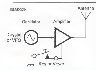
Figure 5.9 — The simplest transmitter consists of the oscillator and amplifier and a means of turning the output signal on and off — the key.
