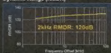
14MHz Band Reciprocal Mixing Dynamic Range (RMDR)
