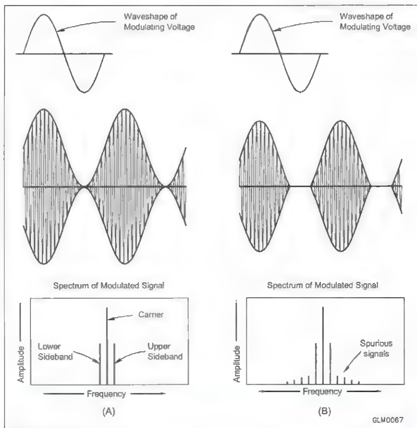
Figure 5.13 — A properly modulated signal at A. The results of overmodulation are visible at B. This distorted signal causes interference on nearby frequencies.
