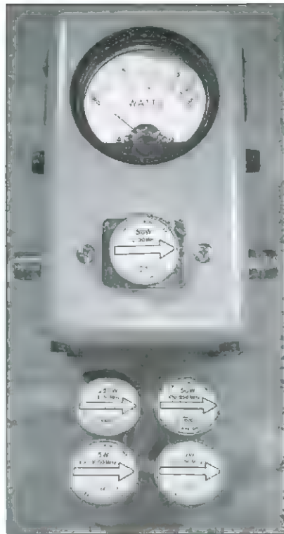
Figure 4.37 — The Bird Model 43 directional wattmeter uses sensing elements designed for a specific frequency range and power level. Forward and reflected power are read by rotating the sensing element. (One sensing element is plugged into the meter, and four other elements for different power levels and frequency ranges are shown below the meter.)
