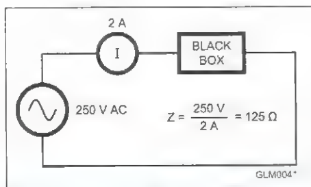
Figure 4.13 — In this circuit we know that the box presents 125 \Omega of impedance (opposition to ac current), but we don't know what's in the box.
