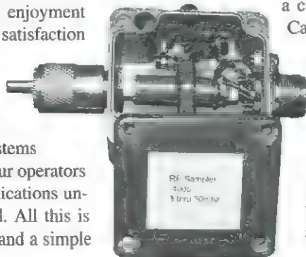
Amateur Radio is unique in that hams are encouraged to build and use their own equipment. This sensing unit for the output power of a transmitter or amplifier, built by Ed Toal, N9MW, is a good example of useful “home-brewing” widespread in ham radio.
