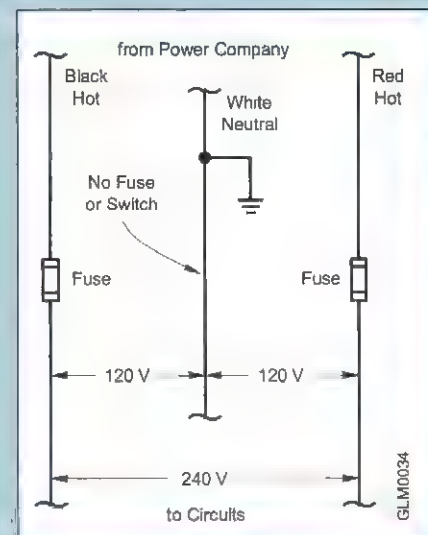
Figure 9.4 — Fuses and circuit breakers should be placed in the hot wire or wires of ac power wiring. Never install a fuse or circuit breaker in the neutral or ground wire of ac wiring. If a neutral or ground wire is disconnected, ac voltage is not removed from the equipment and may still present a shock or fire hazard.
