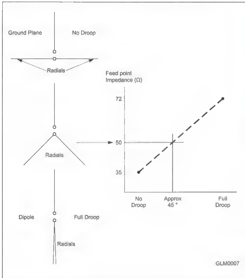
Figure 7.4 — The feed point impedance of a ground-plane antenna with radials perpendicular to the antenna is approximately 35 Ω, resulting in a 1.4:1 SWR with 50-Ω coaxial cable. Drooping or sloping the radials gradually raises the feed point impedance until, with the radials drooped so far as to become the other half of a dipole, feed point impedance becomes 72 Ω. A 50-Ω feed point is reached with radials drooping approximately 45 degrees.
