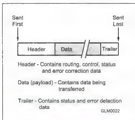
Figure 6.2 — Packet communication systems package data with control and routing information and add error detection information. Each package of header, data, and trailer is called a frame. Different packet protocols use different sets of information and methods of creating the frame.
