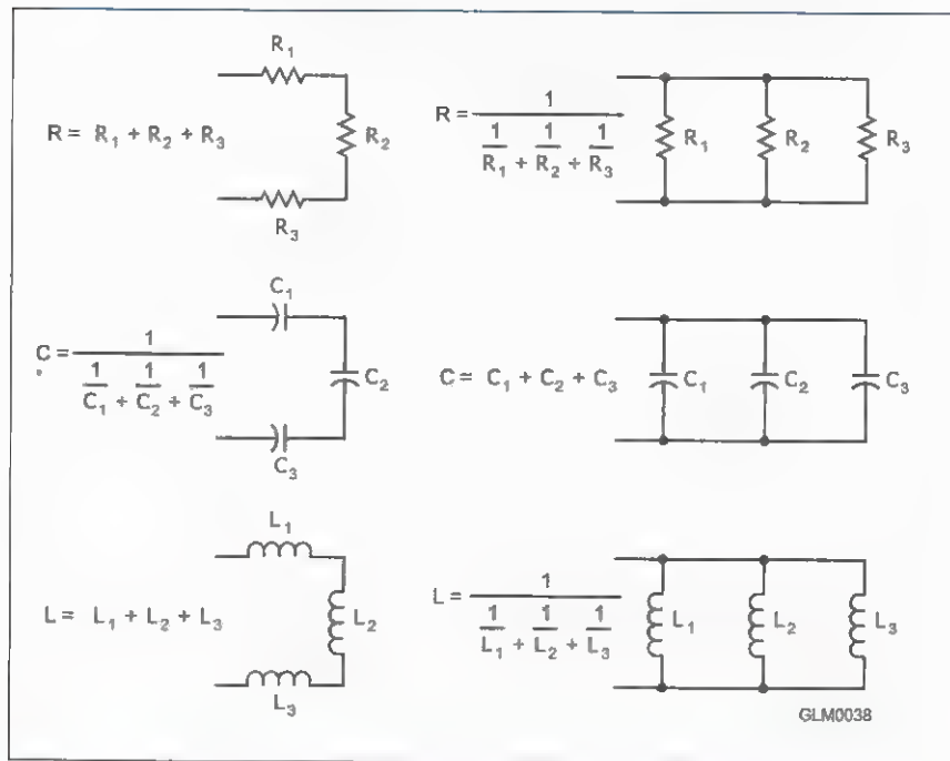
Figure 4.10 — This drawing illustrates how components in series and parallel can be combined into a single equivalent component value.
