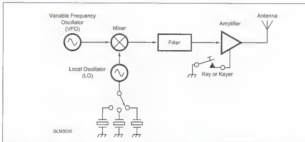
Figure 5.10 — By changing the frequency of the local oscillator (LO), the VFO's output can be shifted from band to band, creating a multiband transmitter.
