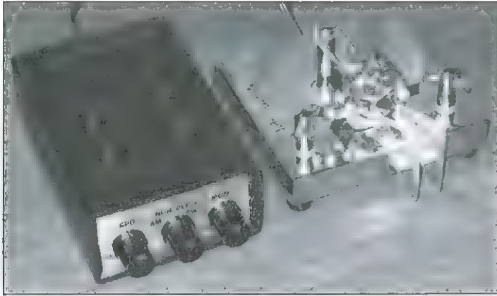
Figure 2.4 — An electronic keyer generates precisely formed and spaced dits and dahs under the control of a paddle. This combination makes it easy to send code at speeds over 15 words per minute (WPM) with much less effort.
