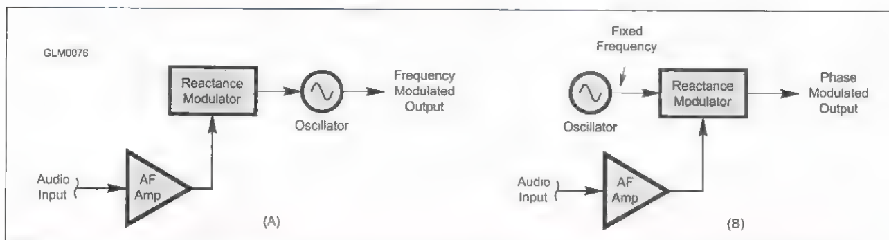
Figure 5.7 — Reactance modulators can be used to create frequency modulation (A) or phase modulation (B).
