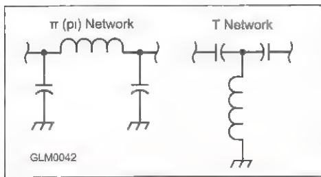
Figure 4.15 — The pi ( \pi ) and T networks are named for the letters that they resemble. The pi network is often used to transform the impedances between transistors or tubes in amplifiers and feed lines. The T network is common in stand-alone “antenna tuners” or “transmatches.”
