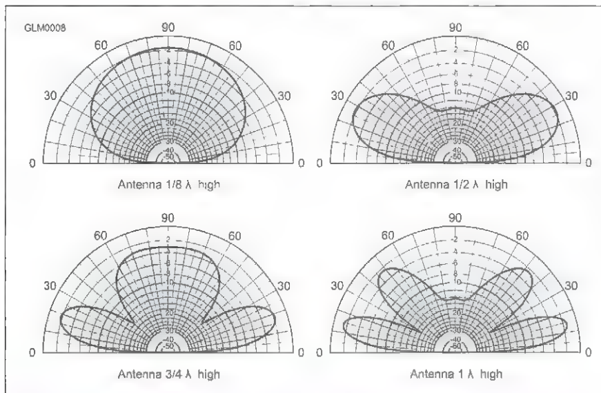
Figure 7.6 — As a low dipole starting at \frac{1}{8} wavelength above ground is raised, the effects of its electrical ground image cause the elevation pattern to flatten out. At multiples of \frac{1}{2} wavelength in height, the pattern has a null in the vertical direction because the direct and reflected signals cancel.
