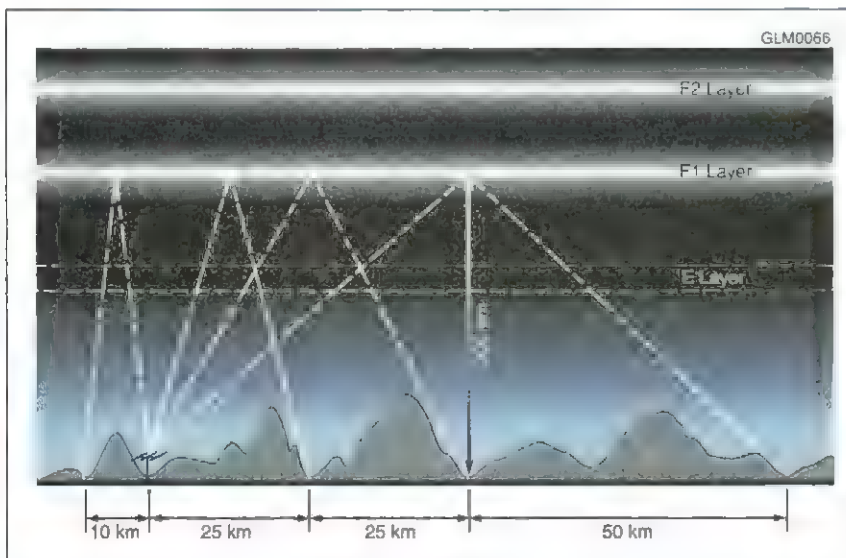
Figure 8.9 — Near vertical incidence sky-wave (NVIS) communications relies on signals below the critical frequency transmitted at high vertical angles. The signals are reflected by the ionosphere back to Earth in the region around the transmitter.
