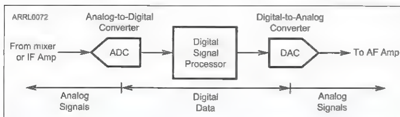
Figure 5.18 — DSP systems use an analog-to-digital converter (ADC) to change the signal to digital data. A special type of microprocessor then performs the mathematical operations on the data to accomplish filtering, noise reduction, or other functions. A digital-to-analog converter (DAC) changes the processed data back to analog form for output as audio.
