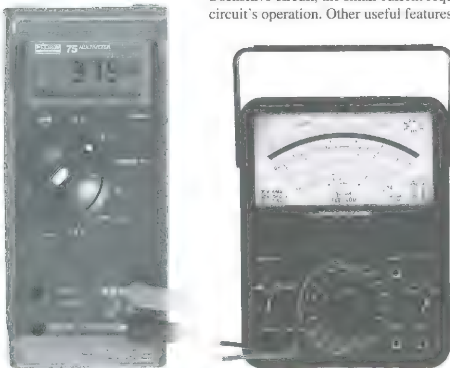
Figure 4.32 — A digital voltmeter (DVM) shown at the left provides precise measurements of voltage, current and resistance. Many models can also act as a frequency counter or component tester. Analog meters (right) are often preferable for tuning and adjustments since the needle's movement makes adjusting for a maximum or minimum quite easy.
