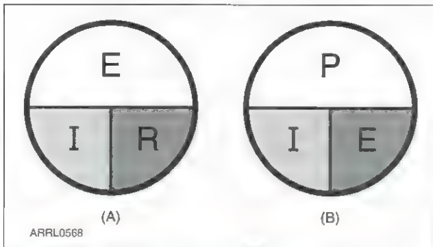
Figure 4.1 — These simple diagrams will help you remember the Ohm's Law relationships and power equations. If you know any two of the quantities, you can find the third by covering up the unknown quantity. The positions of the remaining two symbols show if you have to multiply (side-by-side) or divide (one above the other).
