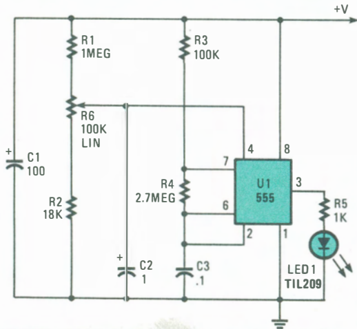
SUPPLY VOLTAGE MONITOR
