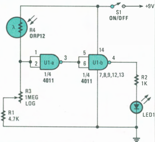
ENLARGER EXPOSURE METER
