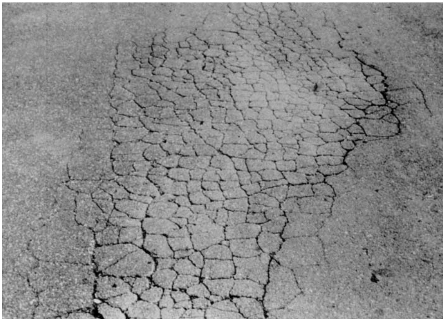
Figure 2.1. Example of alligator cracking
