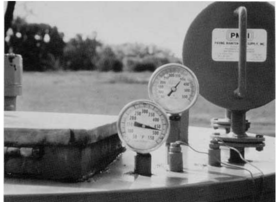
Figure 8.2. Thermometers measuring sealant and oil bath temperature
