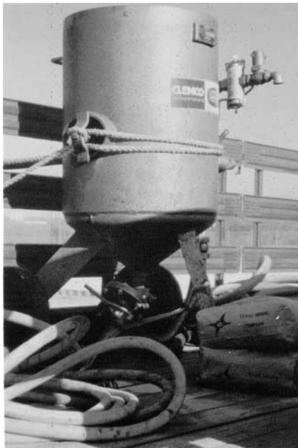
Figure 6.7. Sandblasting equipment
