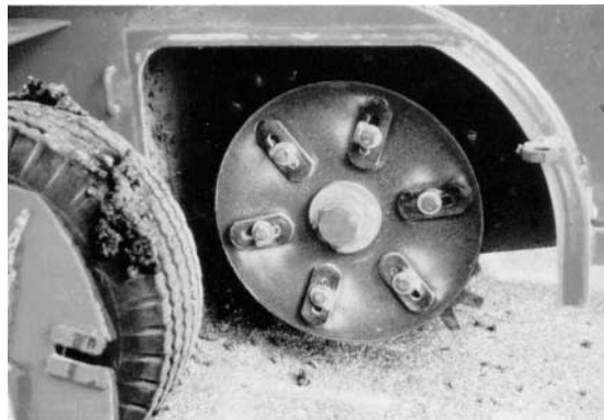
Figure 6.2. Rotary impact router
