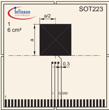
FR4; 80x80x1.5 mm; 35 µm Cu, 5 µm Sn A = 600 mm²; a = 24.49 mm
