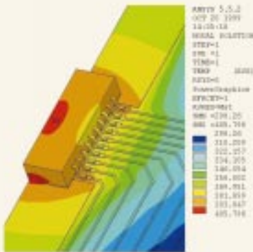
A = 600 mm 2 ; T_a = 298 K; T_{max} = 406 K
