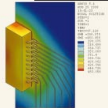
Footprint only; T_a = 298 K; T_{max} = 463 K
