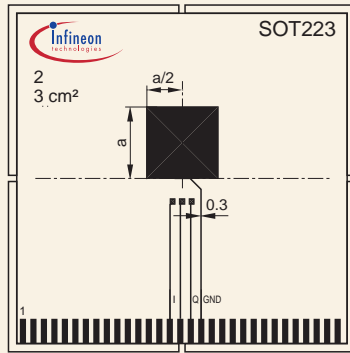
FR4; 80x80x1.5 mm; 35 µm Cu, 5 µm Sn A = 300 mm²; a = 17.32 mm
