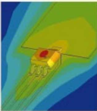
A = 600 mm²; T_a = 298 \text{ K} ; T_{max} = 332 \text{ K}
