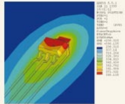
Footprint only; T_a = 298 \text{ K} ; T_{max} = 380 \text{ K}
