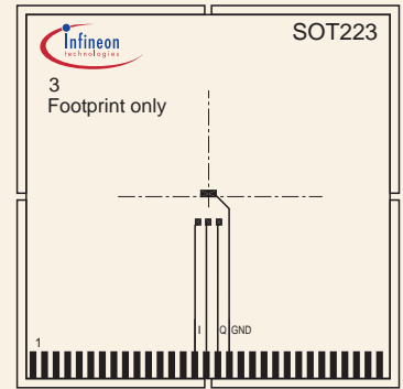
FR4; 80x80x1.5 mm; 35 µm Cu, 5 µm Sn Footprint only
