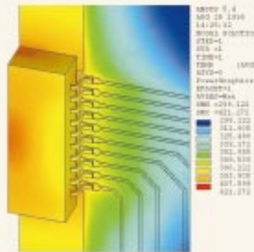
A = 300 mm 2 ; T_a = 298 K; T_{max} = 421 K
