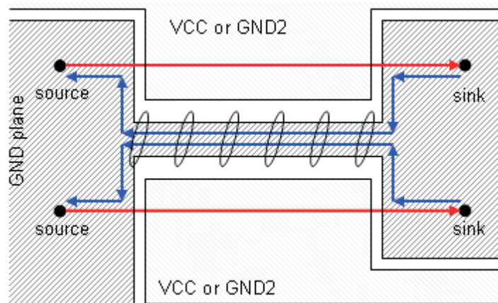
Figure 10. Crosstalk Induced by the Return Current Path
