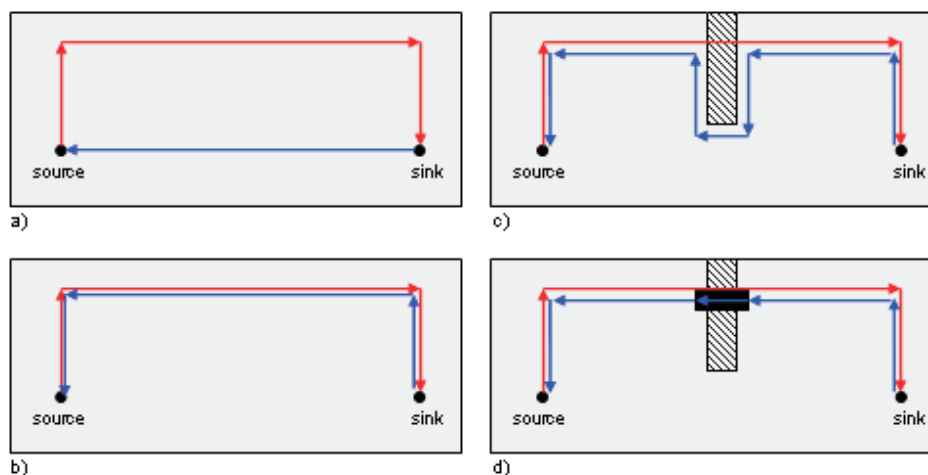
Figure 6. Return Current and Resulting Loop Area
